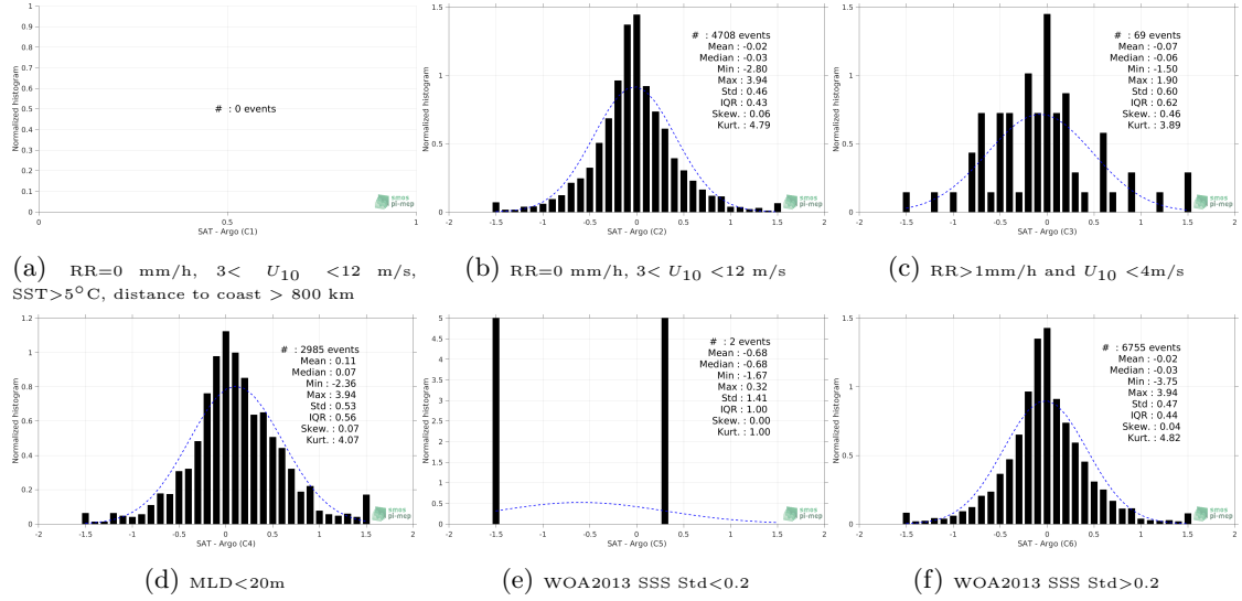
Figure 13: Normalized histogram of \Delta SSS (Aquarius-L4-IPRC-V5-WEEKLY - Argo) for 6 different subdatasets corresponding to: RR=0 mm/h, 3 < U_{10} < 12 m/s, SST > 5^\circ\text{C} , distance to coast > 800 km (a), RR=0 mm/h, 3 < U_{10} < 12 m/s (b), RR > 1 mm/h and U_{10} < 4 m/s (c), MLD < 20 m (d), WOA2013 SSS Std < 0.2 (e), WOA2013 SSS Std > 0.2 (f).
