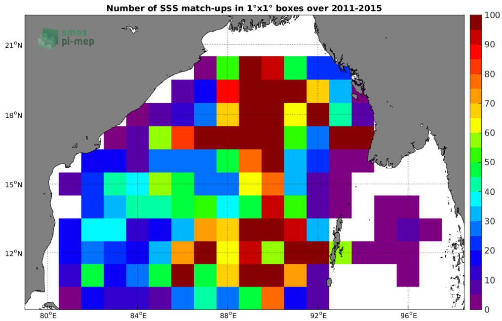
Figure 4: Number of SSS match-ups between Argo SSS and the Aquarius-L4-IPRC-V5-WEEKLY SSS product for the Bay of Bengal Pi-MEP region over 1^\circ \times 1^\circ boxes and for the full satellite product period.
