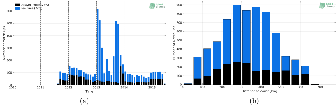
Figure 1: Number of match-ups between Argo and Aquarius-L4-IPRC-V5-WEEKLY SSS as a function of time (a) and as function of the distance to coast (b) over the Bay of Bengal Pi-MEP region and for the full satellite product period.
