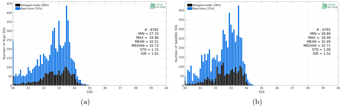
Figure 2: Histograms of SSS from Argo (a) and Aquarius-L4-IPRC-V5-WEEKLY (b) considering all match-up pairs per bins of 0.1 over the Bay of Bengal Pi-MEP region and for the full satellite product period.
