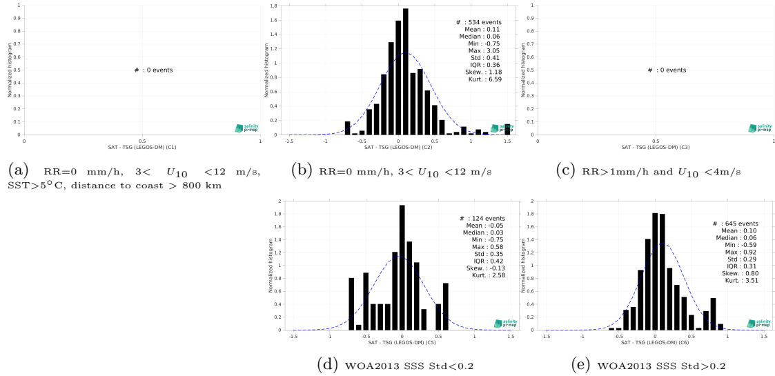
Figure 15: Normalized histogram of \Delta SSS (Aquarius SSS L4 OI v5 - Monthly (IPRC) - TSG (LEGOS-DM)) for 5 different subdatasets corresponding to: RR=0 mm/h, 3 < U_{10} < 12 m/s, SST > 5°C, distance to coast > 800 km (a), RR=0 mm/h, 3 < U_{10} < 12 m/s (b), RR > 1mm/h and U_{10} < 4 m/s (c), WOA2013 SSS Std < 0.2 (d), WOA2013 SSS Std > 0.2 (e).
