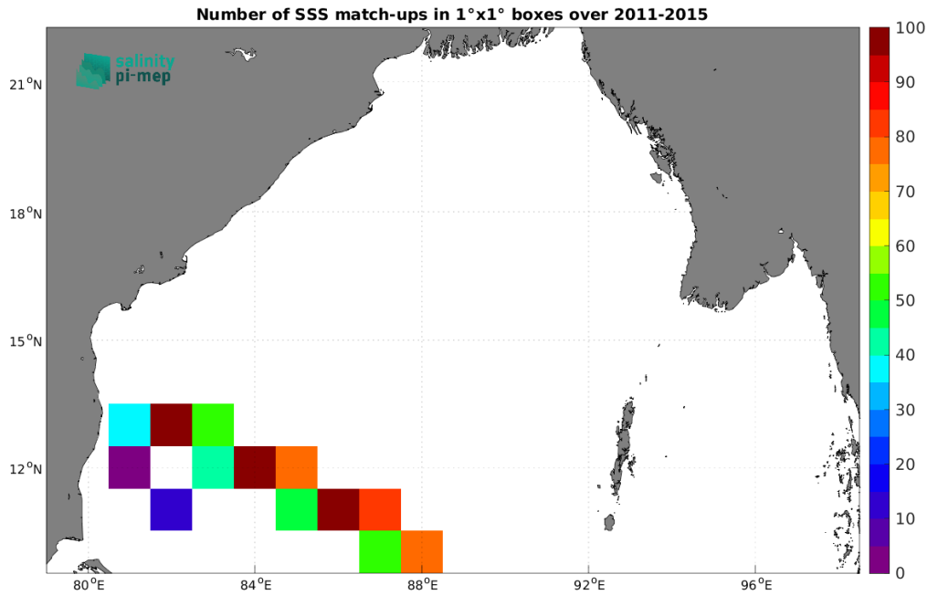
Figure 5: Number of SSS match-ups between TSG (LEGOS-DM) SSS and the Aquarius SSS L4 OI v5 - Monthly (IPRC) SSS product for the Bay of Bengal Pi-MEP region over 1^\circ \times 1^\circ boxes and for the full satellite product period.
