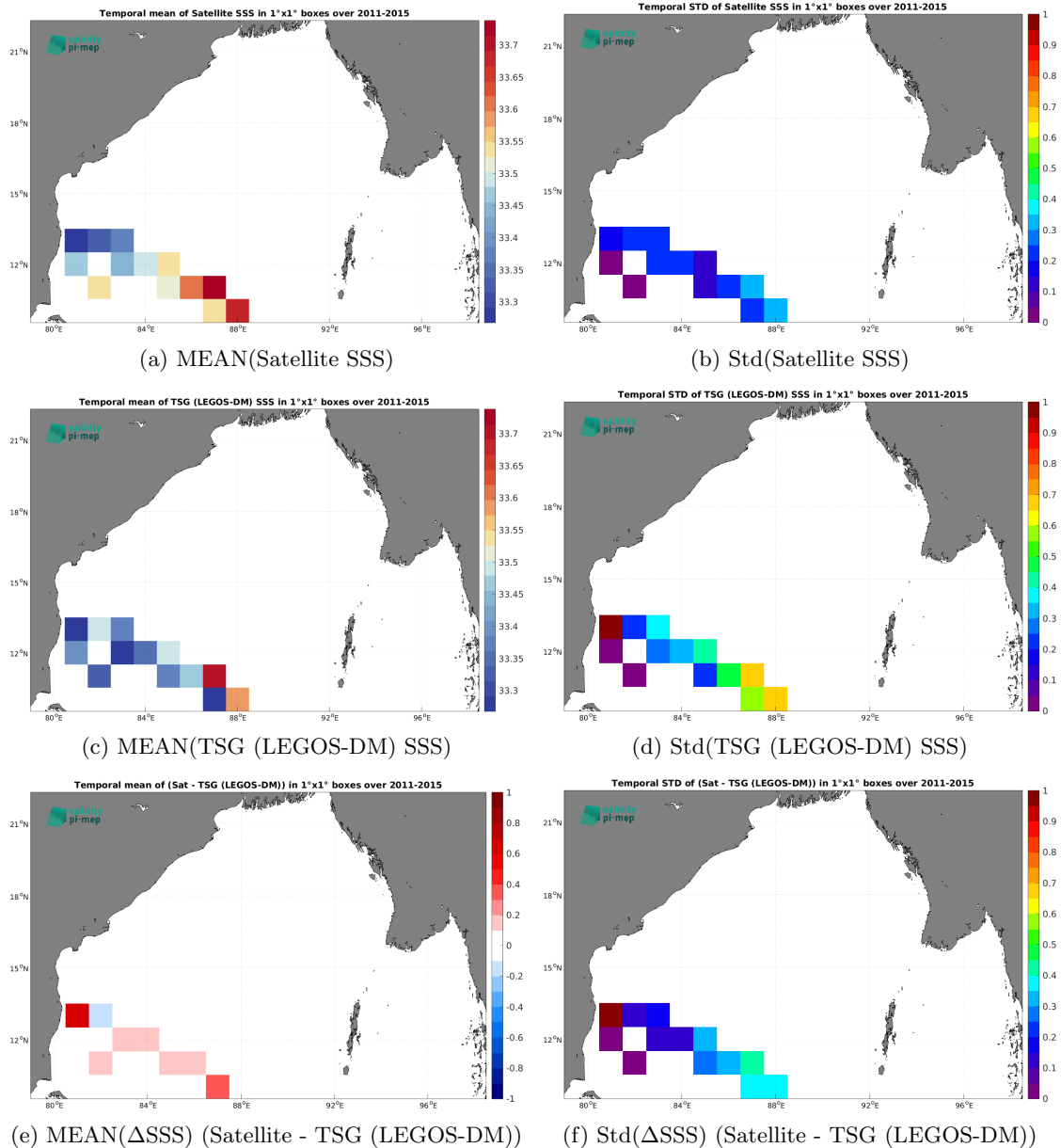
Figure 7: Temporal mean (left) and Std (right) of SSS from Aquarius SSS L4 OI v5 - Monthly (IPRC) (top), TSG (LEGOS-DM) (middle), and of \Delta SSS (Satellite - TSG (LEGOS-DM)). Only match-up pairs are used to generate these maps.
