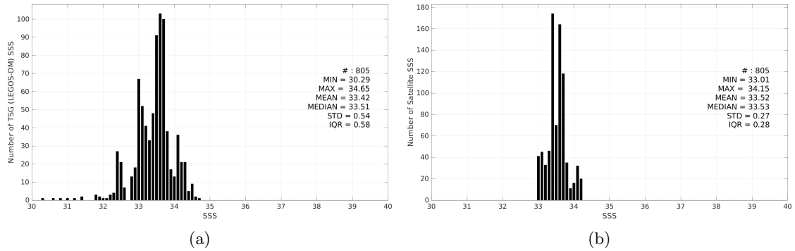
Figure 3: Histograms of SSS from TSG (LEGOS-DM) (a) and Aquarius SSS L4 OI v5 - Monthly (IPRC) (b) considering all match-up pairs per bins of 0.1 over the Bay of Bengal Pi-MEP region and for the full satellite product period.
