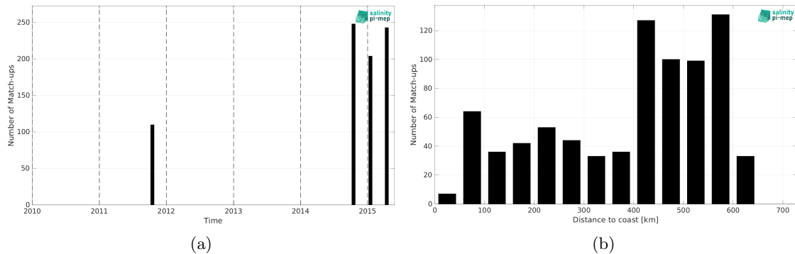
Figure 2: Number of match-ups between TSG (LEGOS-DM) and Aquarius SSS L4 OI v5 - Monthly (IPRC) SSS as a function of time (a) and as function of the distance to coast (b) over the Bay of Bengal Pi-MEP region and for the full satellite product period.
