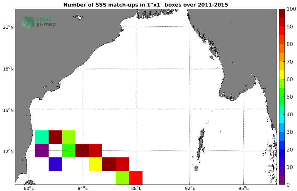
Figure 4: Number of SSS match-ups between TSG (LEGOS-DM) SSS and the Aquarius SSS L4 OI v5 - Monthly (IPRC) SSS product for the Bay of Bengal Pi-MEP region over 1°x1° boxes and for the full satellite product period.
