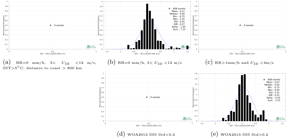
Figure 13: Normalized histogram of \Delta\text{SSS} (Aquarius SSS L4 OI v5 - Monthly (IPRC) - TSG (LEGOS-DM)) for 5 different subdatasets corresponding to: RR=0 mm/h, 3 < U_{10} < 12 m/s, SST > 5^\circ\text{C} , distance to coast > 800 km (a), RR=0 mm/h, 3 < U_{10} < 12 m/s (b), RR > 1 mm/h and U_{10} < 4 m/s (c), WOA2013 SSS Std < 0.2 (d), WOA2013 SSS Std > 0.2 (e).
