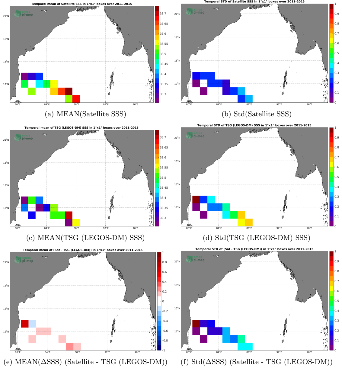
Figure 6: Temporal mean (left) and Std (right) of SSS from Aquarius SSS L4 OI v5 - Monthly (IPRC) (top), TSG (LEGOS-DM) (middle), and of \Delta SSS (Satellite - TSG (LEGOS-DM)). Only match-up pairs are used to generate these maps.
