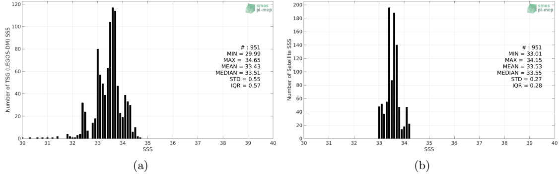
Figure 2: Histograms of SSS from TSG (LEGOS-DM) (a) and Aquarius SSS L4 OI v5 - Monthly (IPRC) (b) considering all match-up pairs per bins of 0.1 over the Bay of Bengal Pi-MEP region and for the full satellite product period.
