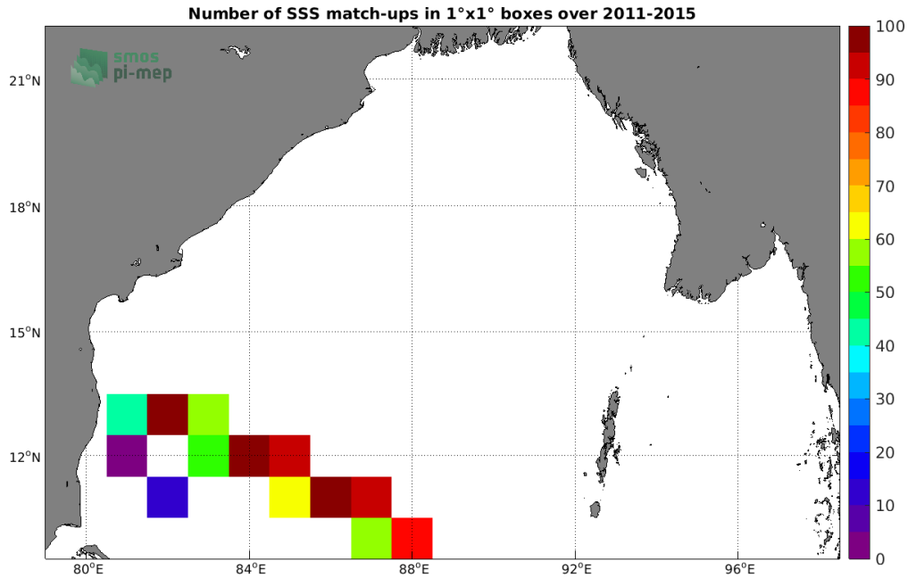
Figure 4: Number of SSS match-ups between TSG (LEGOS-DM) SSS and the Aquarius SSS L4 OI v5 - Monthly (IPRC) SSS product for the Bay of Bengal Pi-MEP region over 1^\circ \times 1^\circ boxes and for the full satellite product period.
