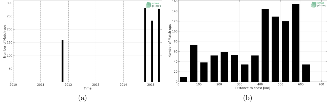
Figure 1: Number of match-ups between TSG (LEGOS-DM) and Aquarius SSS L4 OI v5 - Monthly (IPRC) SSS as a function of time (a) and as function of the distance to coast (b) over the Bay of Bengal Pi-MEP region and for the full satellite product period.
