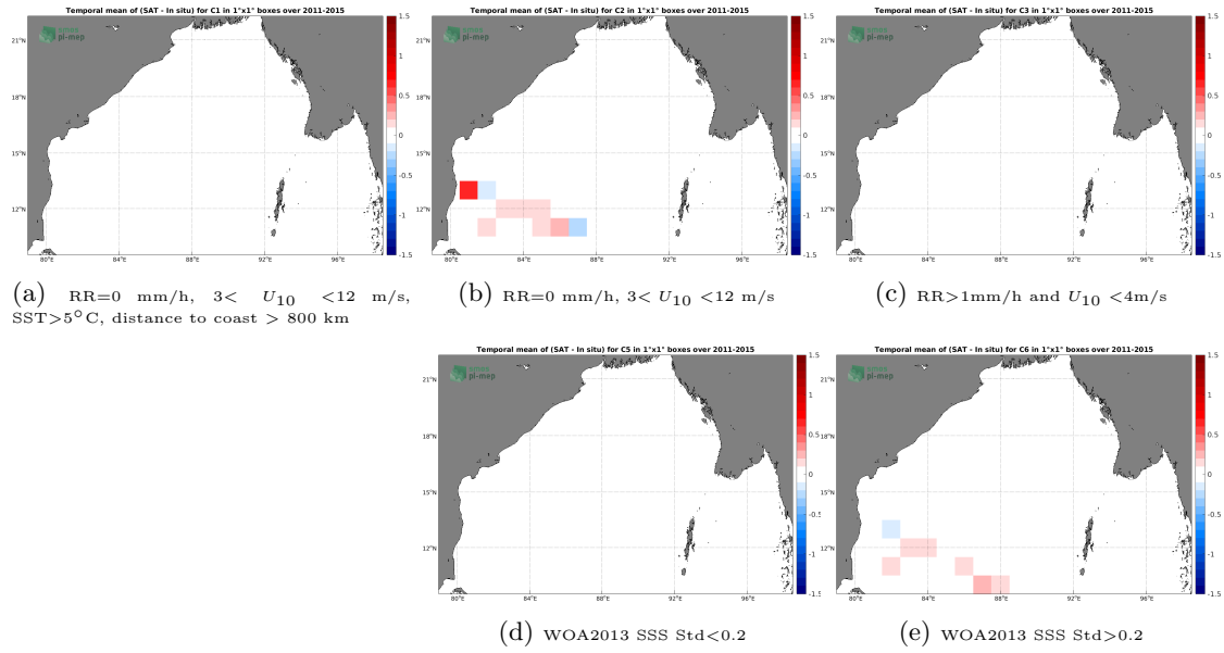
Figure 12: Temporal mean gridded over spatial boxes of size 1^\circ \times 1^\circ of \Delta SSS (Aquarius SSS L4 OI v5 - Monthly (IPRC) - TSG (LEGOS-DM)) for 5 different subdatasets corresponding to: RR=0 mm/h, 3 < U_{10} < 12 m/s, SST >5^\circ\text{C} , distance to coast > 800 km (a), RR=0 mm/h, 3 < U_{10} < 12 m/s (b), RR >1 mm/h and U_{10} < 4 m/s (c), WOA2013 SSS Std <0.2 (d), WOA2013 SSS Std >0.2 (e).
