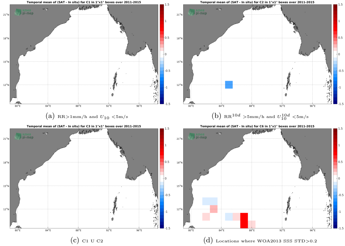
Figure 12: Temporal mean gridded over spatial boxes of size 1^\circ \times 1^\circ of \Delta SSS (Aquarius-L4-IPRC-V5-MONTHLY - TSG-LEGOS-DM) for 4 different subdatasets corresponding to: RR > 1\text{mm/h} and U_{10} < 5\text{m/s} (a), RR^{10d} > 5\text{mm/h} and U_{10}^{10d} < 5\text{m/s} (b), C1 U C2 (c), Locations where WOA2013 SSS STD > 0.2 (d).
