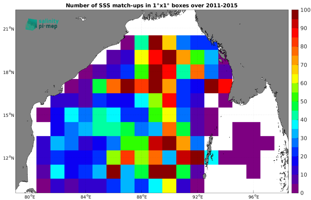
Figure 5: Number of SSS match-ups between Argo SSS and the Aquarius SSS L4 OI v5 - Monthly (IPRC) SSS product for the Bay of Bengal Pi-MEP region over 1^\circ \times 1^\circ boxes and for the full satellite product period.
