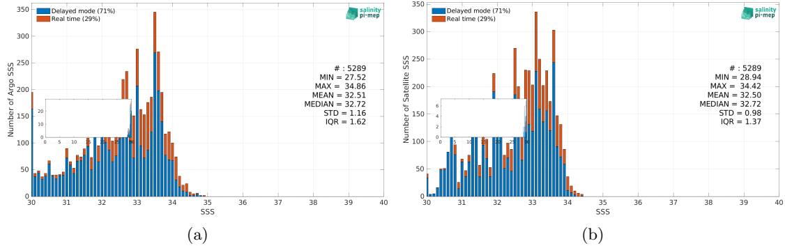
Figure 3: Histograms of SSS from Argo (a) and Aquarius SSS L4 OI v5 - Monthly (IPRC) (b) considering all match-up pairs per bins of 0.1 over the Bay of Bengal Pi-MEP region and for the full satellite product period.
