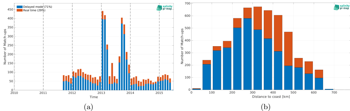
Figure 2: Number of match-ups between Argo and Aquarius SSS L4 OI v5 - Monthly (IPRC) SSS as a function of time (a) and as function of the distance to coast (b) over the Bay of Bengal Pi-MEP region and for the full satellite product period.
