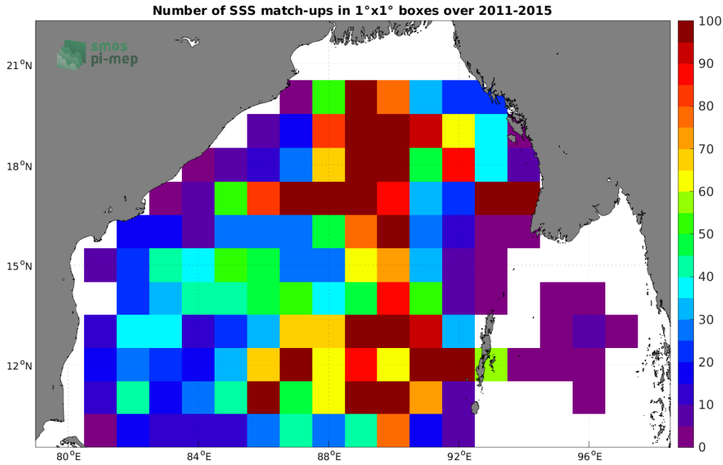
Figure 4: Number of SSS match-ups between Argo SSS and the Aquarius SSS L4 OI v5 - Monthly (IPRC) SSS product for the Bay of Bengal Pi-MEP region over 1^{\circ} \times 1^{\circ} boxes and for the full satellite product period.
