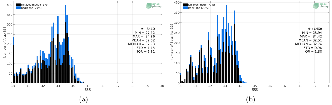
Figure 2: Histograms of SSS from Argo (a) and Aquarius SSS L4 OI v5 - Monthly (IPRC) (b) considering all match-up pairs per bins of 0.1 over the Bay of Bengal Pi-MEP region and for the full satellite product period.
