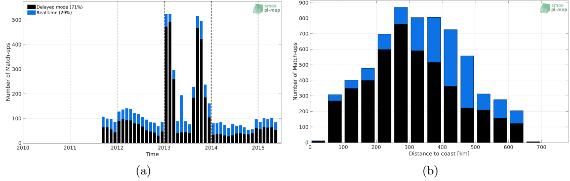
Figure 1: Number of match-ups between Argo and Aquarius SSS L4 OI v5 - Monthly (IPRC) SSS as a function of time (a) and as function of the distance to coast (b) over the Bay of Bengal Pi-MEP region and for the full satellite product period.
