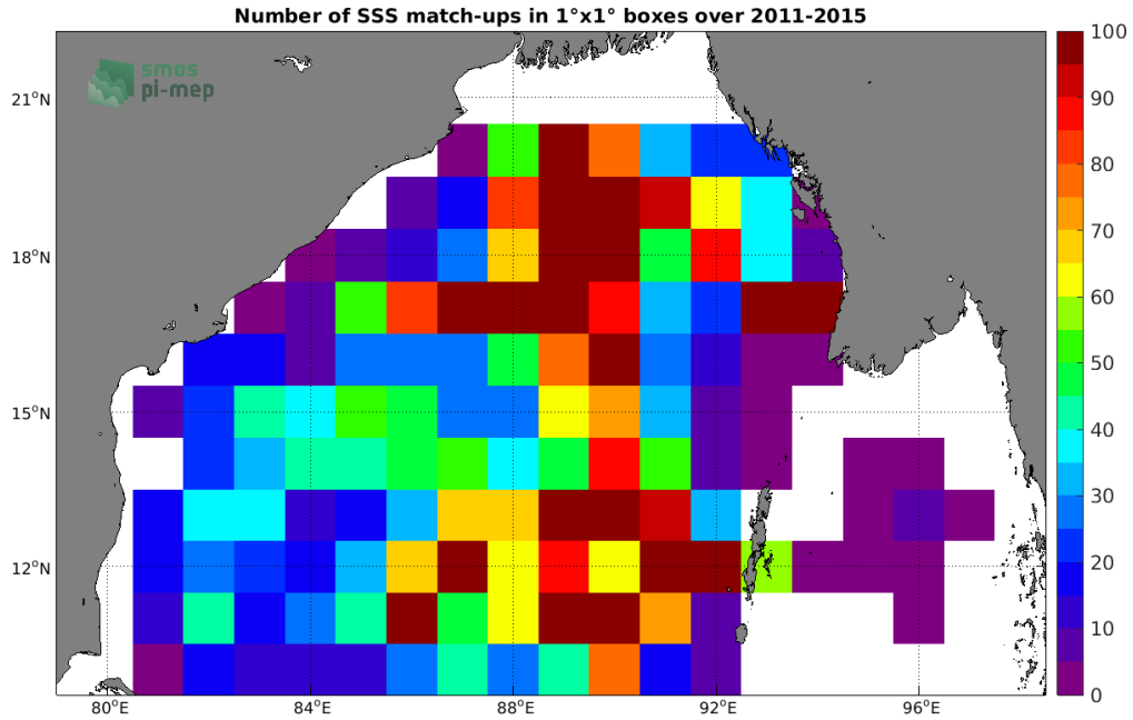
Figure 4: Number of SSS match-ups between Argo SSS and the Aquarius SSS L4 OI v5 - Monthly (IPRC) SSS product for the Bay of Bengal Pi-MEP region over 1^\circ \times 1^\circ boxes and for the full satellite product period.
