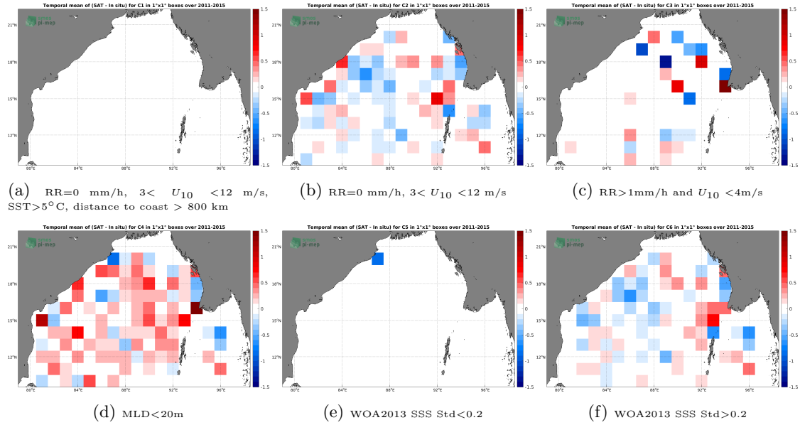
Figure 12: Temporal mean gridded over spatial boxes of size 1^\circ \times 1^\circ of \Delta SSS (Aquarius SSS L4 OI v5 - Monthly (IPRC) - Argo) for 6 different subdatasets corresponding to: RR=0 mm/h, 3 < U_{10} < 12 m/s, SST > 5^\circ C , distance to coast > 800 km (a), RR=0 mm/h, 3 < U_{10} < 12 m/s (b), RR > 1 mm/h and U_{10} < 4 m/s (c), MLD < 20 m (d), WOA2013 SSS Std < 0.2 (e), WOA2013 SSS Std > 0.2 (f).
