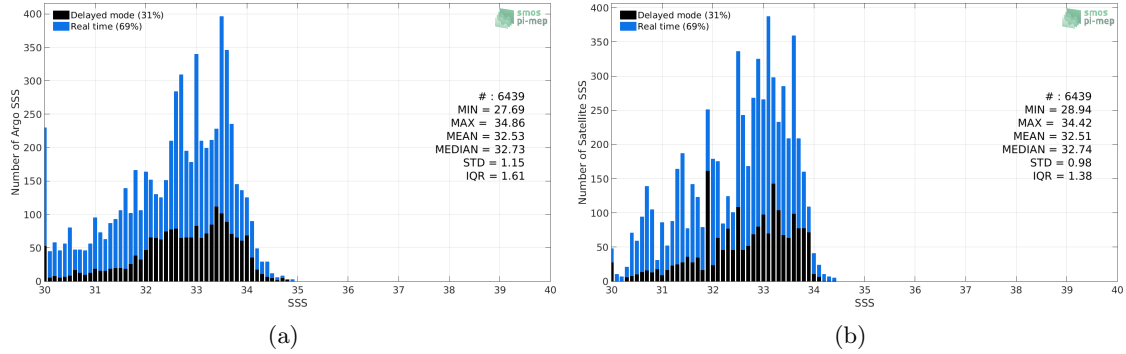
Figure 2: Histograms of SSS from Argo (a) and Aquarius-L4-IPRC-V5-MONTHLY (b) considering all match-up pairs per bins of 0.1 over the Bay of Bengal Pi-MEP region and for the full satellite product period.
