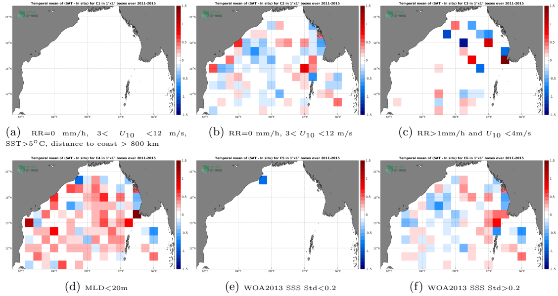
Figure 12: Temporal mean gridded over spatial boxes of size 1^\circ \times 1^\circ of \Delta SSS (Aquarius-L4-IPRC-V5-MONTHLY - Argo) for 6 different subdatasets corresponding to: RR=0 mm/h, 3 < U_{10} < 12 m/s, SST >5^\circ C, distance to coast > 800 km (a), RR=0 mm/h, 3 < U_{10} < 12 m/s (b), RR >1 mm/h and U_{10} < 4 m/s (c), MLD <20 m (d), WOA2013 SSS Std <0.2 (e), WOA2013 SSS Std >0.2 (f).
