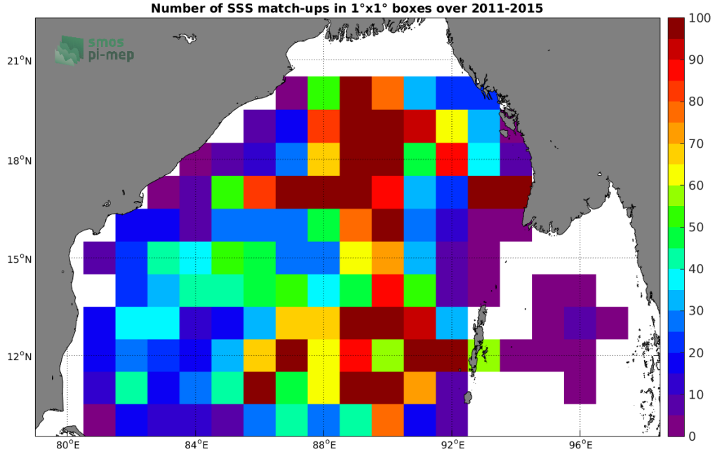
Figure 4: Number of SSS match-ups between Argo SSS and the Aquarius-L4-IPRC-V5-MONTHLY SSS product for the Bay of Bengal Pi-MEP region over 1^\circ \times 1^\circ boxes and for the full satellite product period.
