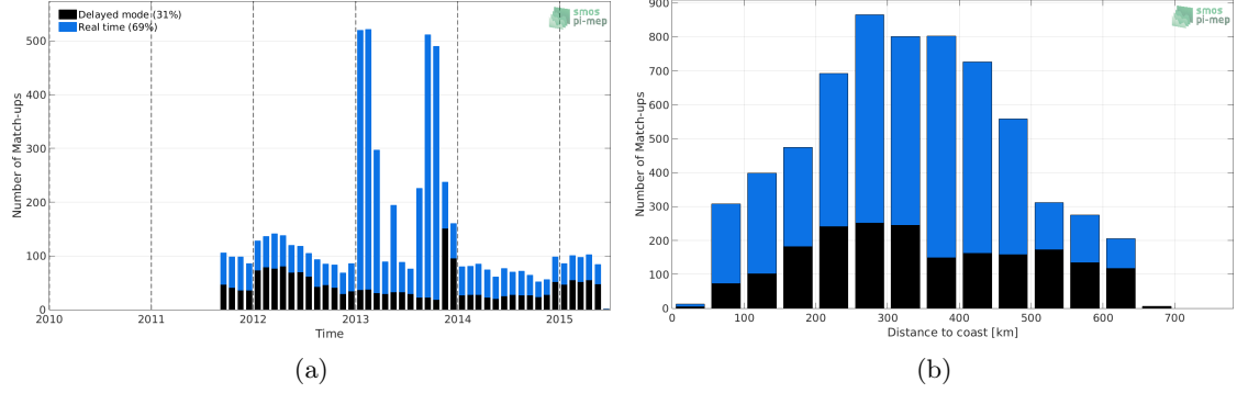
Figure 1: Number of match-ups between Argo and Aquarius-L4-IPRC-V5-MONTHLY SSS as a function of time (a) and as function of the distance to coast (b) over the Bay of Bengal Pi-MEP region and for the full satellite product period.
