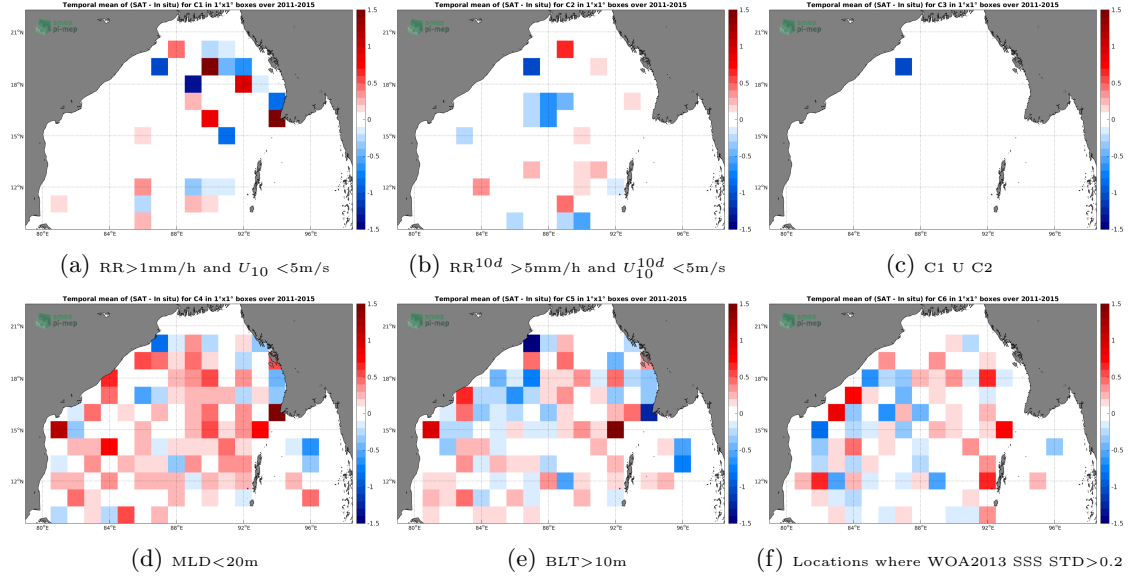
Figure 12: Temporal mean gridded over spatial boxes of size 1^\circ \times 1^\circ of \Delta\text{SSS} (Aquarius-L4-IPRC-V5-MONTHLY - Argo) for 6 different subdatasets corresponding to: \text{RR} > 1\text{mm/h} and U_{10} < 5\text{m/s} (a), \text{RR}^{10d} > 5\text{mm/h} and U_{10}^{10d} < 5\text{m/s} (b), C1 U C2 (c), \text{MLD} < 20\text{m} (d), \text{BLT} > 10\text{m} (e), Locations where WOA2013 SSS STD > 0.2 (f).
