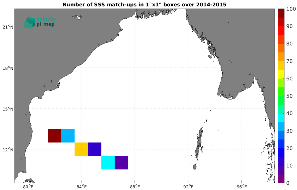
Figure 5: Number of SSS match-ups between TSG (LEGOS-DM) SSS and the Aquarius SSS L3 OR v5 - 7-Day running (NASA-GSFC) SSS product for the Bay of Bengal Pi-MEP region over 1^\circ \times 1^\circ boxes and for the full satellite product period.
