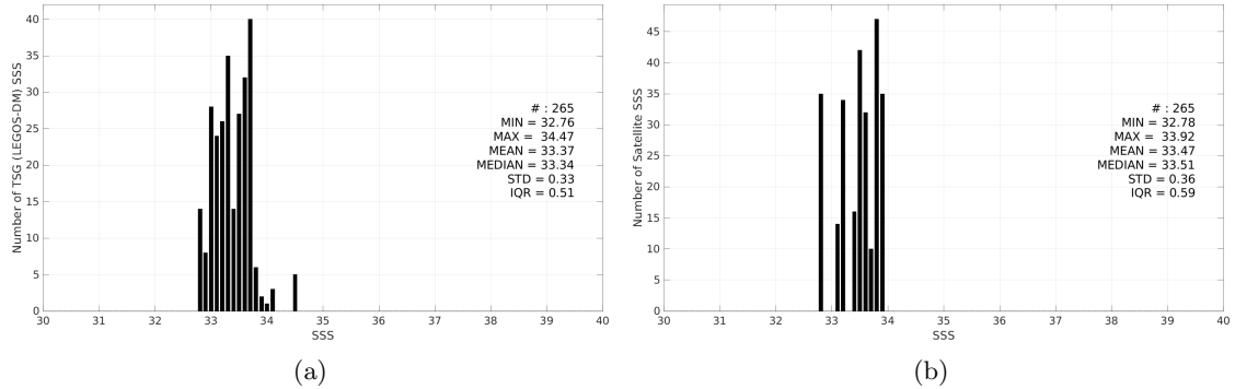
Figure 3: Histograms of SSS from TSG (LEGOS-DM) (a) and Aquarius SSS L3 OR v5 - 7-Day running (NASA-GSFC) (b) considering all match-up pairs per bins of 0.1 over the Bay of Bengal Pi-MEP region and for the full satellite product period.
