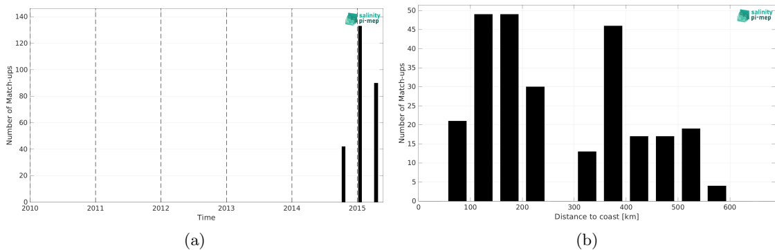
Figure 2: Number of match-ups between TSG (LEGOS-DM) and Aquarius SSS L3 OR v5 - 7-Day running (NASA-GSFC) SSS as a function of time (a) and as function of the distance to coast (b) over the Bay of Bengal Pi-MEP region and for the full satellite product period.
