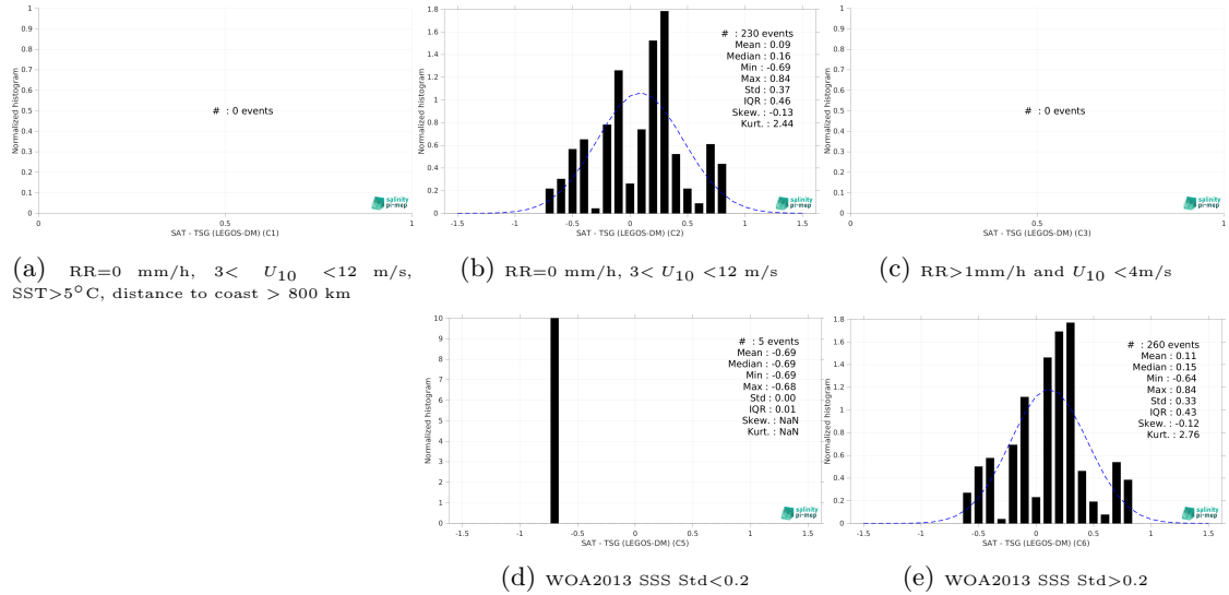
Figure 15: Normalized histogram of \Delta SSS (Aquarius SSS L3 OR v5 - 7-Day running (NASA-GSFC) - TSG (LEGOS-DM)) for 5 different subdatasets corresponding to: RR=0 mm/h, 3 < U_{10} < 12 m/s, SST > 5°C, distance to coast > 800 km (a), RR=0 mm/h, 3 < U_{10} < 12 m/s (b), RR > 1mm/h and U_{10} < 4 m/s (c), WOA2013 SSS Std < 0.2 (d), WOA2013 SSS Std > 0.2 (e).
