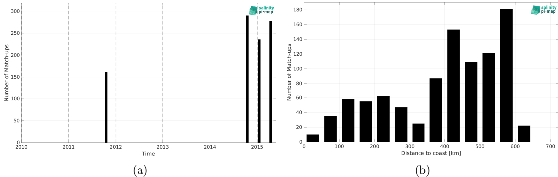
Figure 1: Number of match-ups between TSG (LEGOS-DM) and Aquarius SSS L3 OR v5 - 7-Day running (NASA-GSFC) SSS as a function of time (a) and as function of the distance to coast (b) over the Bay of Bengal Pi-MEP region and for the full satellite product period.
