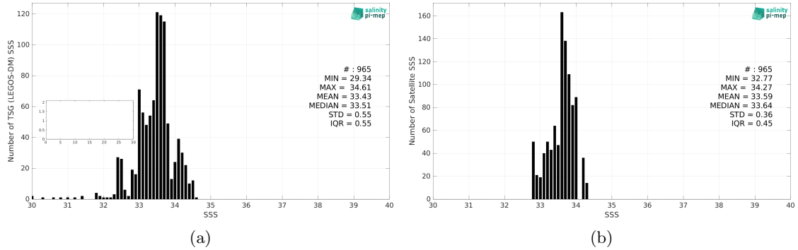
Figure 2: Histograms of SSS from TSG (LEGOS-DM) (a) and Aquarius SSS L3 OR v5 - 7-Day running (NASA-GSFC) (b) considering all match-up pairs per bins of 0.1 over the Bay of Bengal Pi-MEP region and for the full satellite product period.
