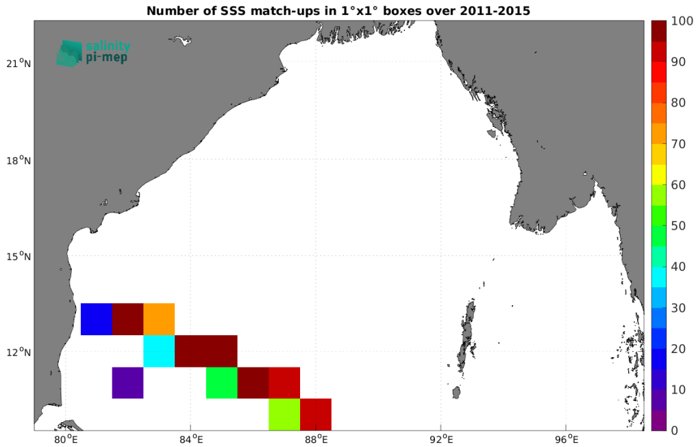
Figure 4: Number of SSS match-ups between TSG (LEGOS-DM) SSS and the Aquarius SSS L3 OR v5 - 7-Day running (NASA-GSFC) SSS product for the Bay of Bengal Pi-MEP region over 1^\circ \times 1^\circ boxes and for the full satellite product period.
