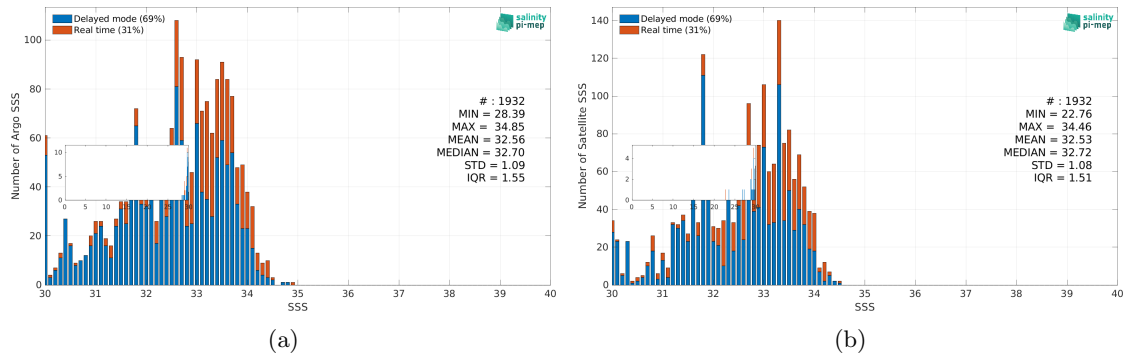
Figure 3: Histograms of SSS from Argo (a) and Aquarius SSS L3 OR v5 - 7-Day running (NASA-GSFC) (b) considering all match-up pairs per bins of 0.1 over the Bay of Bengal Pi-MEP region and for the full satellite product period.
