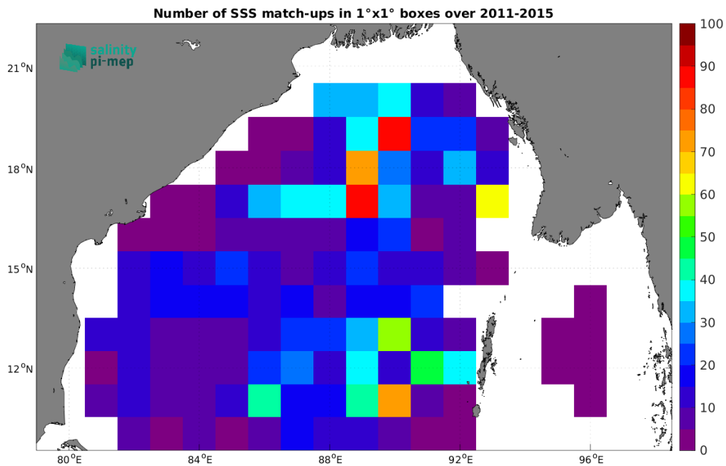
Figure 5: Number of SSS match-ups between Argo SSS and the Aquarius SSS L3 OR v5 - 7-Day running (NASA-GSFC) SSS product for the Bay of Bengal Pi-MEP region over 1^\circ \times 1^\circ boxes and for the full satellite product period.
