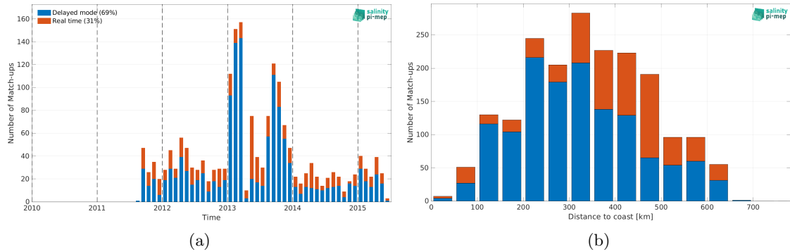
Figure 2: Number of match-ups between Argo and Aquarius SSS L3 OR v5 - 7-Day running (NASA-GSFC) SSS as a function of time (a) and as function of the distance to coast (b) over the Bay of Bengal Pi-MEP region and for the full satellite product period.
