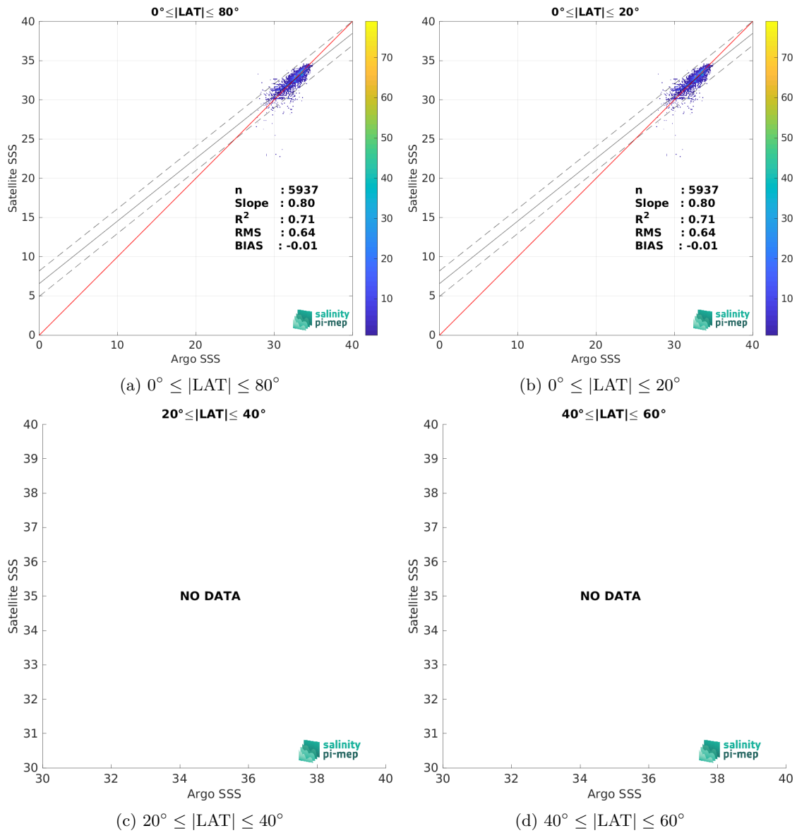
Figure 9: Contour maps of the concentration of Aquarius SSS L3 OR v5 - 7-Day running (NASA-GSFC) SSS ( y -axis) versus Argo SSS ( x -axis) at match-up pairs for different latitude bands. For each plot, the red line shows x=y . The black thin and dashed lines indicate a linear fit through the data cloud and the \pm 95\% confidence levels, respectively. The number match-up pairs n , the slope and R^2 coefficient of the linear fit, the root mean square (RMS) and the mean bias between satellite and in situ data are indicated for each latitude band in each plots.
