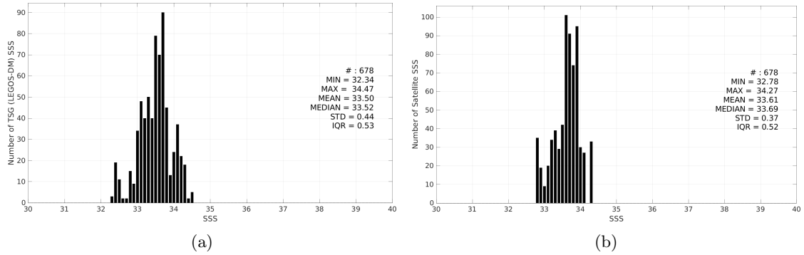
Figure 3: Histograms of SSS from TSG (LEGOS-DM) (a) and Aquarius SSS L3 OR v5 - 7-Day running - Rain mask (NASA-GSFC) (b) considering all match-up pairs per bins of 0.1 over the Bay of Bengal Pi-MEP region and for the full satellite product period.
