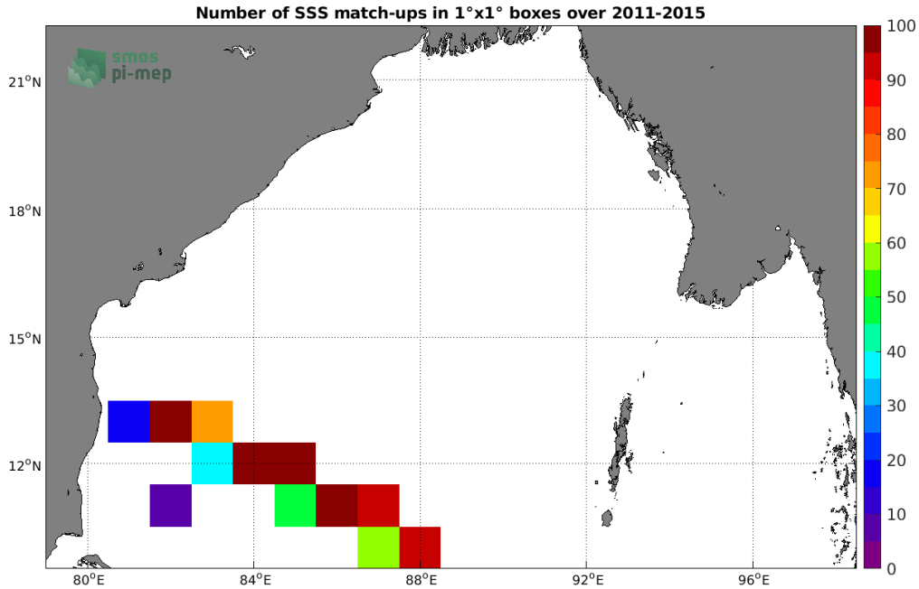
Figure 4: Number of SSS match-ups between TSG (LEGOS-DM) SSS and the Aquarius SSS L3 OR v5 - 7-Day running - Rain mask (NASA-GSFC) SSS product for the Bay of Bengal Pi-MEP region over 1°x1° boxes and for the full satellite product period.
