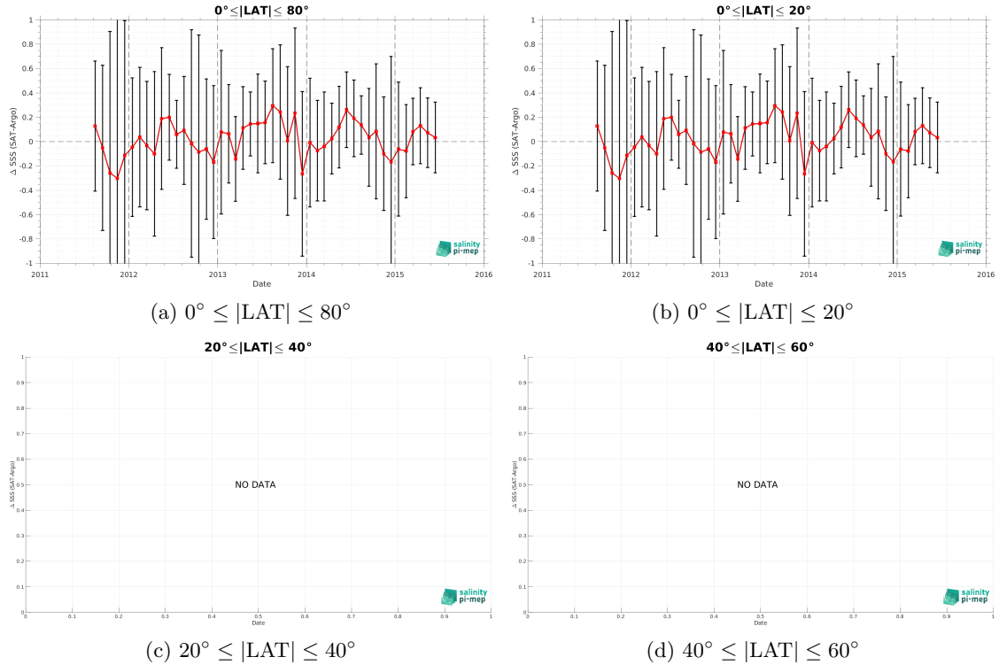
Figure 11: Monthly median (red curves) of \Delta SSS (Satellite - Argo) and \pm 1 Std (black vertical thick bars) as function of time for all the collected Pi-MEP match-up pairs estimated over the Bay of Bengal Pi-MEP region and for the full satellite product period are shown for different latitude bands: (a) 80^\circ\text{S}-80^\circ\text{N} , (b) 20^\circ\text{S}-20^\circ\text{N} , (c) 40^\circ\text{S}-20^\circ\text{S} and 20^\circ\text{N}-40^\circ\text{N} and (d) 60^\circ\text{S}-40^\circ\text{S} and 40^\circ\text{N}-60^\circ\text{N} .
