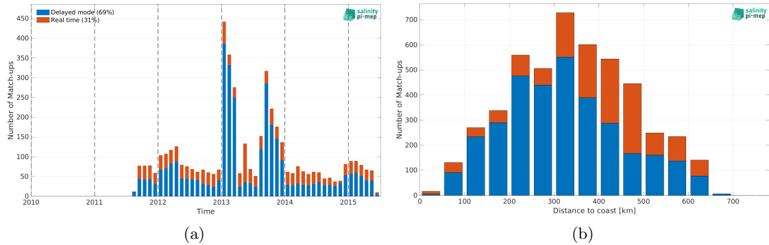
Figure 2: Number of match-ups between Argo and Aquarius SSS L3 OR v5 - 7-Day running - Rain mask (NASA-GSFC) SSS as a function of time (a) and as function of the distance to coast (b) over the Bay of Bengal Pi-MEP region and for the full satellite product period.
