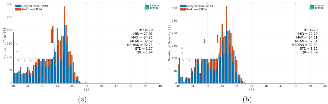
Figure 3: Histograms of SSS from Argo (a) and Aquarius SSS L3 OR v5 - 7-Day running - Rain mask (NASA-GSFC) (b) considering all match-up pairs per bins of 0.1 over the Bay of Bengal Pi-MEP region and for the full satellite product period.
