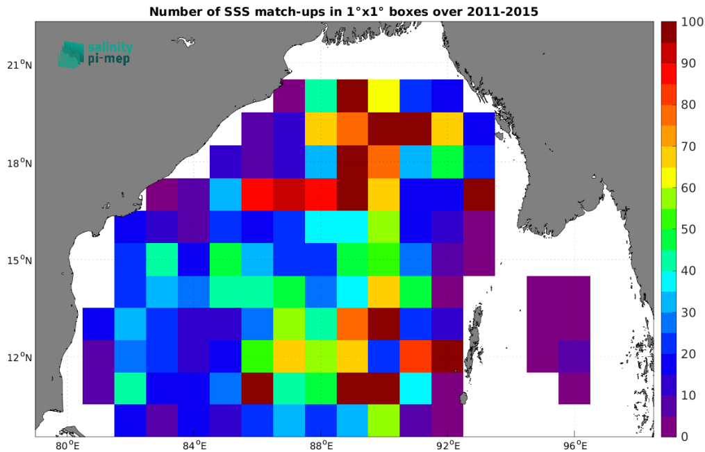
Figure 5: Number of SSS match-ups between Argo SSS and the Aquarius SSS L3 OR v5 - 7-Day running - Rain mask (NASA-GSFC) SSS product for the Bay of Bengal Pi-MEP region over 1^\circ \times 1^\circ boxes and for the full satellite product period.
