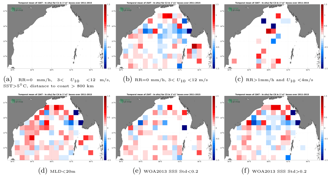
Figure 12: Temporal mean gridded over spatial boxes of size 1^{\circ}\times 1^{\circ} of \Delta\text{SSS} (Aquarius SSS L3 OR v5 - 7-Day running - Rain mask (NASA-GSFC) - Argo) for 6 different subdatasets corresponding to:RR=0 mm/h, 3 < U_{10} < 12 m/s, SST >5^{\circ}\text{C} , distance to coast > 800 km (a), RR=0 mm/h, 3 < U_{10} < 12 m/s (b), RR >1\text{mm/h} and U_{10} < 4\text{m/s} (c),MLD <20\text{m} (d),WOA2013 SSS Std <0.2 (e),WOA2013 SSS Std >0.2 (f).
