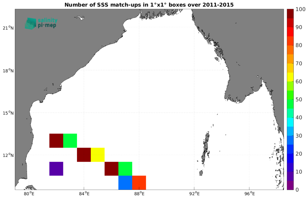
Figure 5: Number of SSS match-ups between TSG (LEGOS-DM) SSS and the Aquarius SSS L3 OR v5 - Monthly (NASA-GSFC) SSS product for the Bay of Bengal Pi-MEP region over 1^\circ \times 1^\circ boxes and for the full satellite product period.
