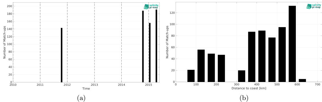
Figure 2: Number of match-ups between TSG (LEGOS-DM) and Aquarius SSS L3 OR v5 - Monthly (NASA-GSFC) SSS as a function of time (a) and as function of the distance to coast (b) over the Bay of Bengal Pi-MEP region and for the full satellite product period.
