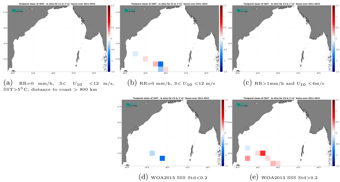
Figure 14: Temporal mean gridded over spatial boxes of size 1^\circ \times 1^\circ of \Delta\text{SSS} (Aquarius SSS L3 OR v5 - Monthly (NASA-GSFC) - TSG (LEGOS-DM)) for 5 different subdatasets corresponding to:RR=0 mm/h, 3 < U_{10} < 12 m/s, SST >5^\circ\text{C} , distance to coast > 800 km (a), RR=0 mm/h, 3 < U_{10} < 12 m/s (b), RR >1 mm/h and U_{10} < 4 m/s (c), WOA2013 SSS Std <0.2 (d), WOA2013 SSS Std >0.2 (e).
