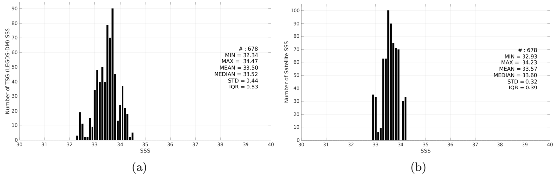
Figure 3: Histograms of SSS from TSG (LEGOS-DM) (a) and Aquarius SSS L3 OR v5 - Monthly (NASA-GSFC) (b) considering all match-up pairs per bins of 0.1 over the Bay of Bengal Pi-MEP region and for the full satellite product period.
