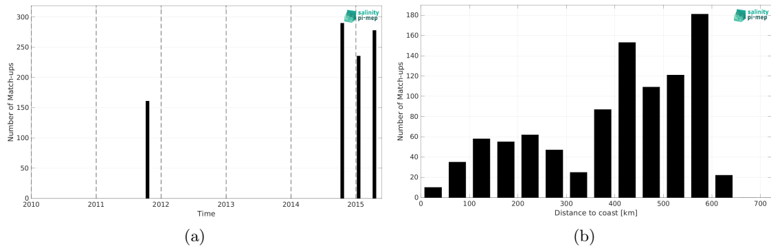
Figure 1: Number of match-ups between TSG (LEGOS-DM) and Aquarius SSS L3 OR v5 - Monthly (NASA-GSFC) SSS as a function of time (a) and as function of the distance to coast (b) over the Bay of Bengal Pi-MEP region and for the full satellite product period.
