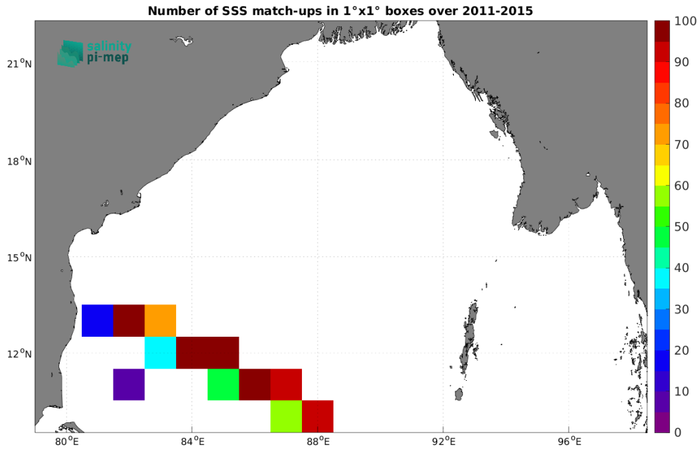
Figure 4: Number of SSS match-ups between TSG (LEGOS-DM) SSS and the Aquarius SSS L3 OR v5 - Monthly (NASA-GSFC) SSS product for the Bay of Bengal Pi-MEP region over 1^\circ \times 1^\circ boxes and for the full satellite product period.
