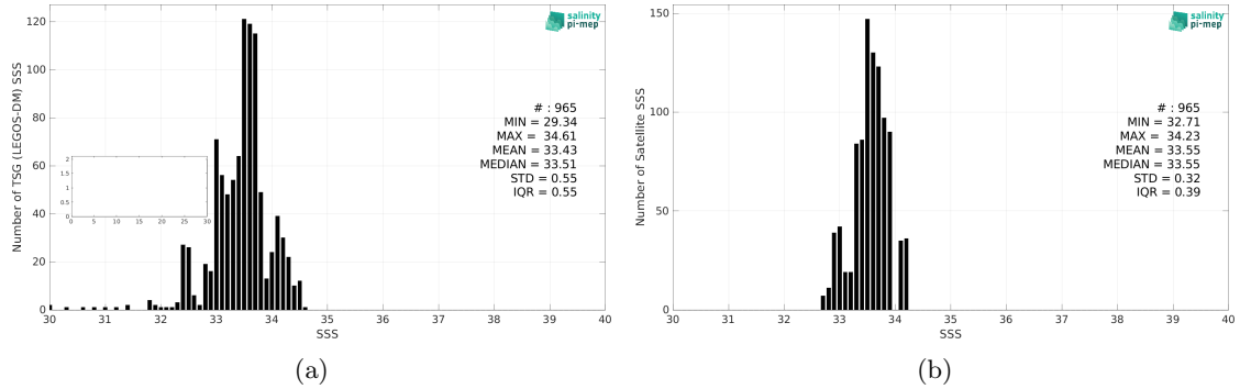
Figure 2: Histograms of SSS from TSG (LEGOS-DM) (a) and Aquarius SSS L3 OR v5 - Monthly (NASA-GSFC) (b) considering all match-up pairs per bins of 0.1 over the Bay of Bengal Pi-MEP region and for the full satellite product period.
