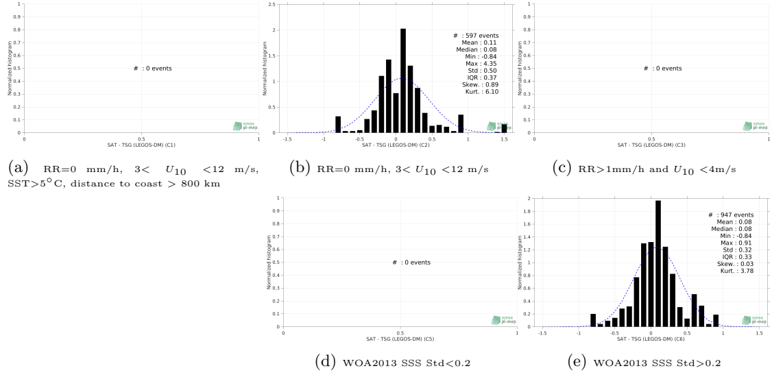
Figure 13: Normalized histogram of \Delta\text{SSS} (Aquarius SSS L3 OR v5 - Monthly (NASA-GSFC) - TSG (LEGOS-DM)) for 5 different subdatasets corresponding to: RR=0 mm/h, 3 < U_{10} < 12 m/s, SST > 5^\circ\text{C} , distance to coast > 800 km (a), RR=0 mm/h, 3 < U_{10} < 12 m/s (b), RR > 1\text{mm/h} and U_{10} < 4\text{m/s} (c), WOA2013 SSS \text{Std} < 0.2 (d), WOA2013 SSS \text{Std} > 0.2 (e).
