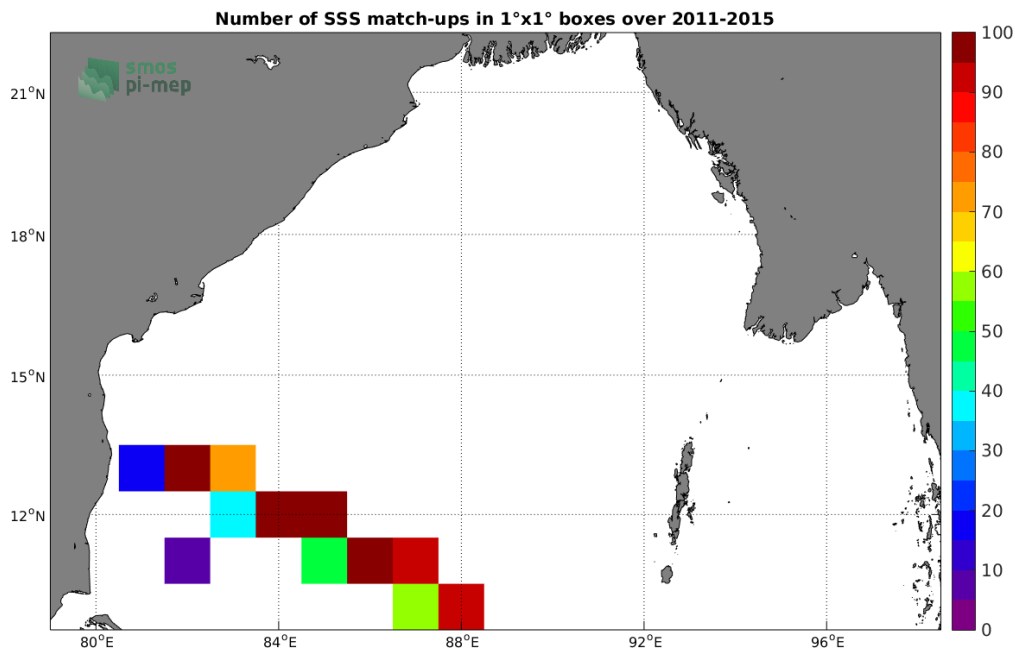
Figure 4: Number of SSS match-ups between TSG-LEGOS-DM SSS and the Aquarius-L3-OR-V5-MONTHLY-1DEG SSS product for the Bay of Bengal Pi-MEP region over 1°x1° boxes and for the full satellite product period.
