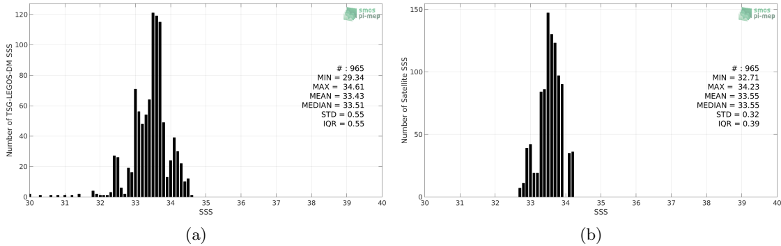
Figure 2: Histograms of SSS from TSG-LEGOS-DM (a) and Aquarius-L3-OR-V5-MONTHLY-1DEG (b) considering all match-up pairs per bins of 0.1 over the Bay of Bengal Pi-MEP region and for the full satellite product period.
