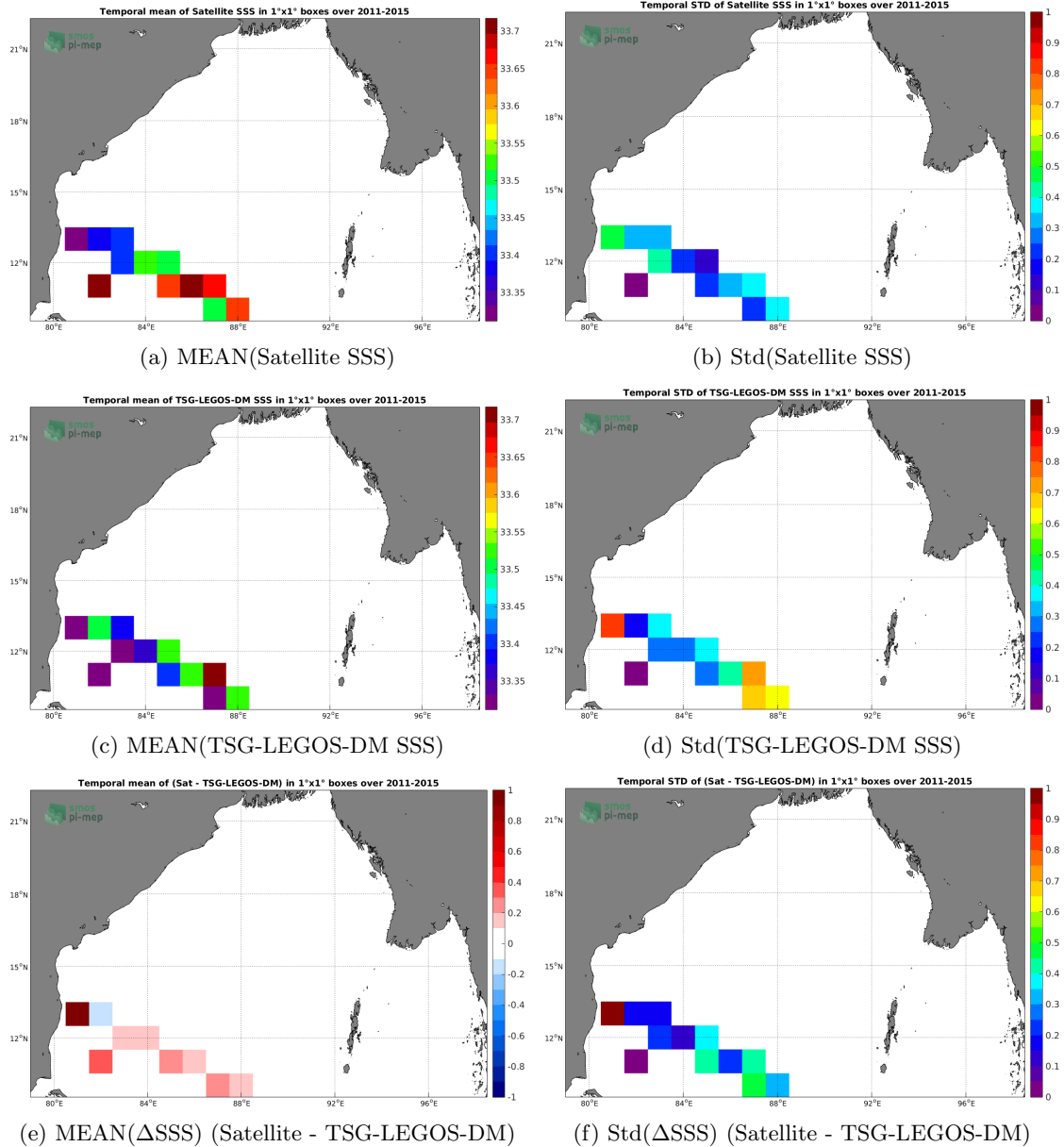
Figure 6: Temporal mean (left) and Std (right) of SSS from Aquarius-L3-OR-V5-MONTHLY-1DEG (top), TSG-LEGOS-DM (middle), and of \Delta SSS (Satellite - TSG-LEGOS-DM). Only match-up pairs are used to generate these maps.
