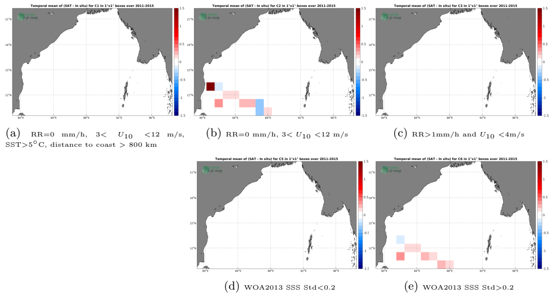
Figure 12: Temporal mean gridded over spatial boxes of size 1^\circ \times 1^\circ of \Delta SSS (Aquarius-L3-OR-V5-MONTHLY-1DEG - TSG-LEGOS-DM) for 5 different subdatasets corresponding to:RR=0 mm/h, 3 < U_{10} < 12 m/s, SST > 5^\circ\text{C} , distance to coast > 800 km (a), RR=0 mm/h, 3 < U_{10} < 12 m/s (b), RR > 1 mm/h and U_{10} < 4 m/s (c), WOA2013 SSS Std < 0.2 (d), WOA2013 SSS Std > 0.2 (e).
