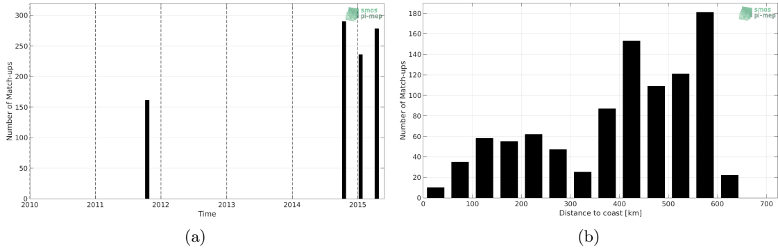
Figure 1: Number of match-ups between TSG-LEGOS-DM and Aquarius-L3-OR-V5-MONTHLY-1DEG SSS as a function of time (a) and as function of the distance to coast (b) over the Bay of Bengal Pi-MEP region and for the full satellite product period.
