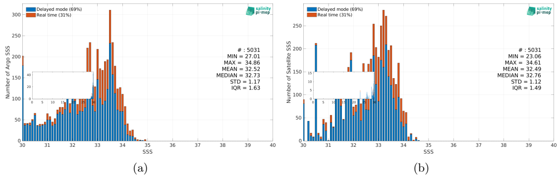
Figure 3: Histograms of SSS from Argo (a) and Aquarius SSS L3 OR v5 - Monthly (NASA-GSFC) (b) considering all match-up pairs per bins of 0.1 over the Bay of Bengal Pi-MEP region and for the full satellite product period.
