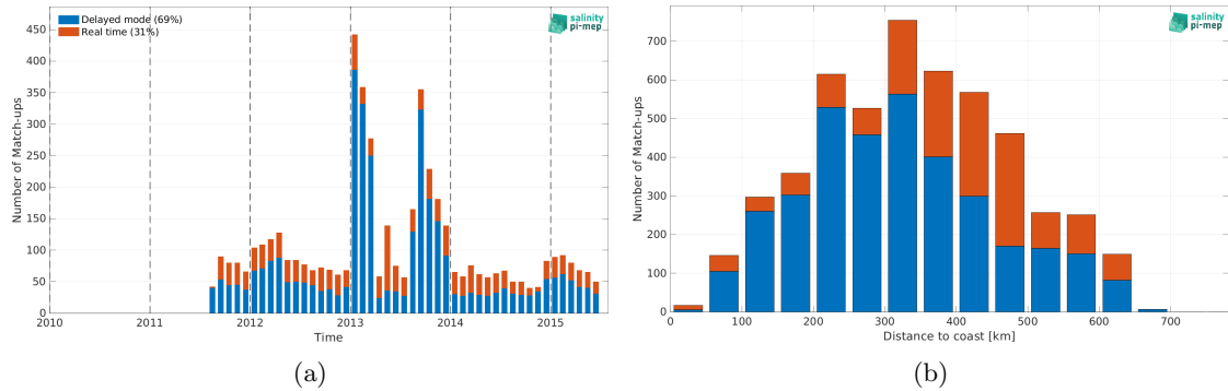
Figure 2: Number of match-ups between Argo and Aquarius SSS L3 OR v5 - Monthly (NASA-GSFC) SSS as a function of time (a) and as function of the distance to coast (b) over the Bay of Bengal Pi-MEP region and for the full satellite product period.
