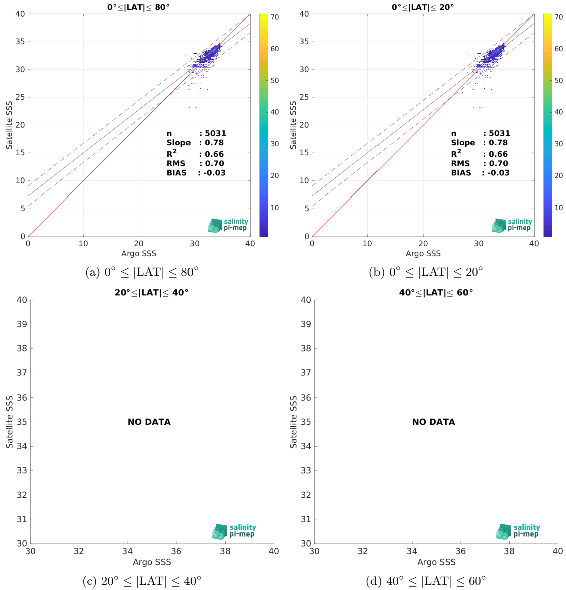
Figure 10: Contour maps of the concentration of Aquarius SSS L3 OR v5 - Monthly (NASA-GSFC) SSS ( y -axis) versus Argo SSS ( x -axis) at match-up pairs for different latitude bands. For each plot, the red line shows x=y . The black thin and dashed lines indicate a linear fit through the data cloud and the \pm 95\% confidence levels, respectively. The number match-up pairs n , the slope and R^2 coefficient of the linear fit, the root mean square (RMS) and the mean bias between satellite and in situ data are indicated for each latitude band in each plots.
