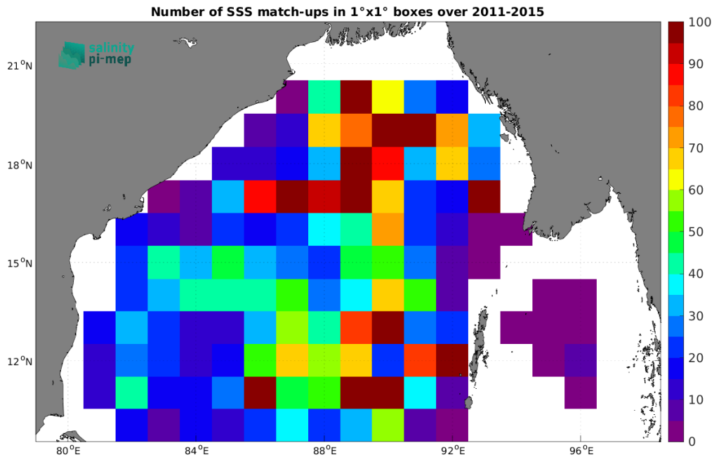
Figure 5: Number of SSS match-ups between Argo SSS and the Aquarius SSS L3 OR v5 - Monthly (NASA-GSFC) SSS product for the Bay of Bengal Pi-MEP region over 1^\circ \times 1^\circ boxes and for the full satellite product period.
