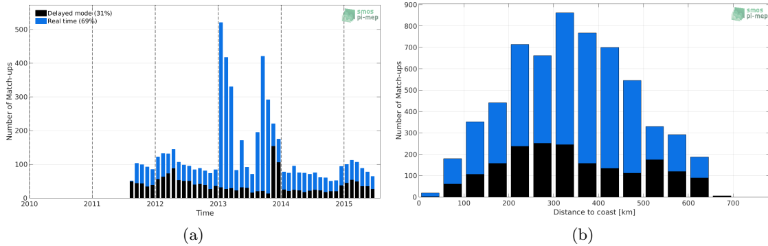
Figure 1: Number of match-ups between Argo and Aquarius-L3-OR-V5-MONTHLY-1DEG SSS as a function of time (a) and as function of the distance to coast (b) over the Bay of Bengal Pi-MEP region and for the full satellite product period.
