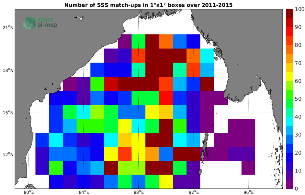
Figure 4: Number of SSS match-ups between Argos SSS and the Aquarius-L3-OR-V5-MONTHLY-1DEG SSS product for the Bay of Bengal Pi-MEP region over 1°x1° boxes and for the full satellite product period.
