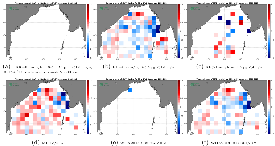
Figure 12: Temporal mean gridded over spatial boxes of size 1°x1° of \Delta SSS (Aquarius-L3-OR-V5-MONTHLY-1DEG - Argo) for 6 different subdatasets corresponding to:RR=0 mm/h, 3 < U_{10} < 12 m/s, SST>5°C, distance to coast > 800 km (a), RR=0 mm/h, 3 < U_{10} < 12 m/s (b), RR>1mm/h and U_{10} < 4 m/s (c),MLD<20m (d),WOA2013 SSS Std<0.2 (e),WOA2013 SSS Std>0.2 (f).
