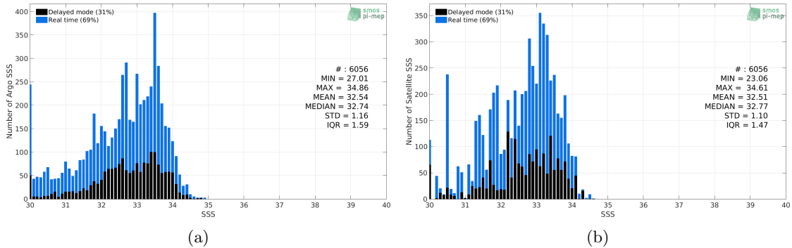
Figure 2: Histograms of SSS from Argo (a) and Aquarius-L3-OR-V5-MONTHLY-1DEG (b) considering all match-up pairs per bins of 0.1 over the Bay of Bengal Pi-MEP region and for the full satellite product period.
