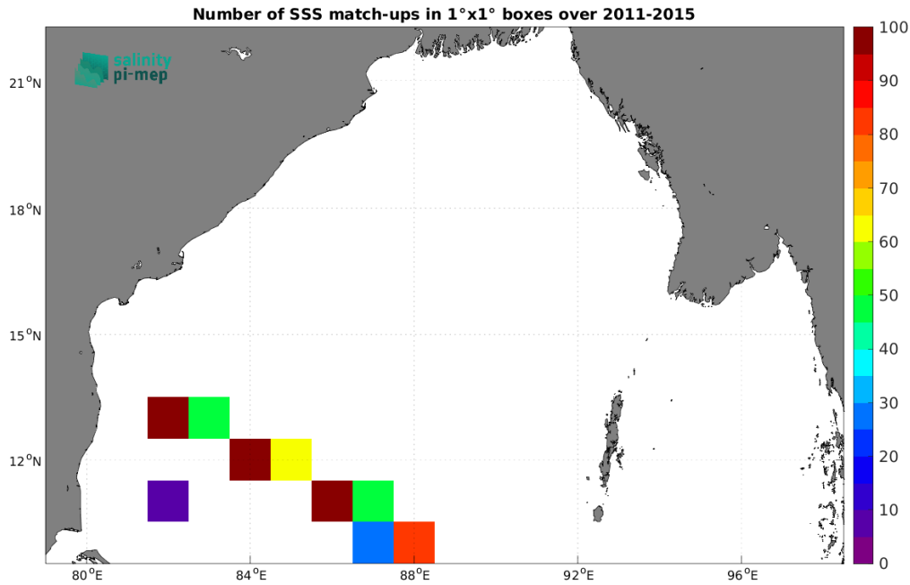
Figure 5: Number of SSS match-ups between TSG (LEGOS-DM) SSS and the Aquarius SSS L3 OR v5 - Monthly - Rain mask (NASA-GSFC) SSS product for the Bay of Bengal Pi-MEP region over 1^\circ \times 1^\circ boxes and for the full satellite product period.
