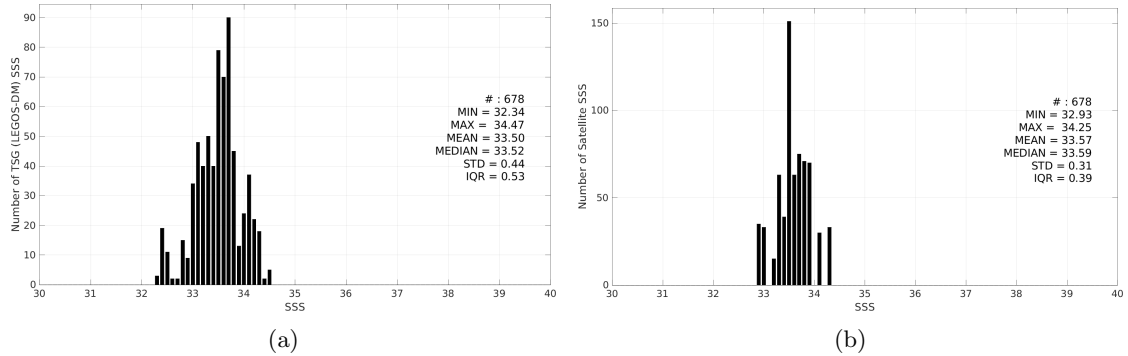
Figure 3: Histograms of SSS from TSG (LEGOS-DM) (a) and Aquarius SSS L3 OR v5 - Monthly - Rain mask (NASA-GSFC) (b) considering all match-up pairs per bins of 0.1 over the Bay of Bengal Pi-MEP region and for the full satellite product period.
