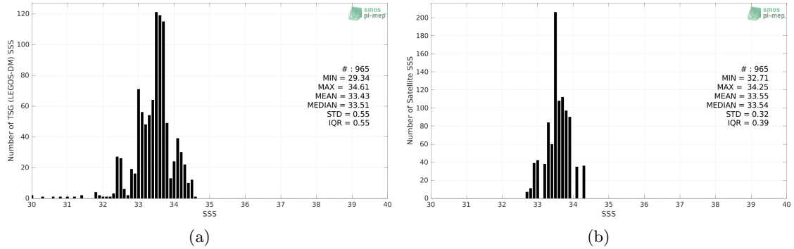
Figure 2: Histograms of SSS from TSG (LEGOS-DM) (a) and Aquarius SSS L3 OR v5 - Monthly - Rain mask (NASA-GSFC) (b) considering all match-up pairs per bins of 0.1 over the Bay of Bengal Pi-MEP region and for the full satellite product period.
