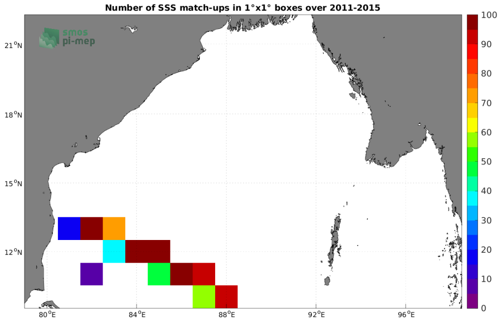
Figure 4: Number of SSS match-ups between TSG (LEGOS-DM) SSS and the Aquarius SSS L3 OR v5 - Monthly - Rain mask (NASA-GSFC) SSS product for the Bay of Bengal Pi-MEP region over 1^\circ \times 1^\circ boxes and for the full satellite product period.
