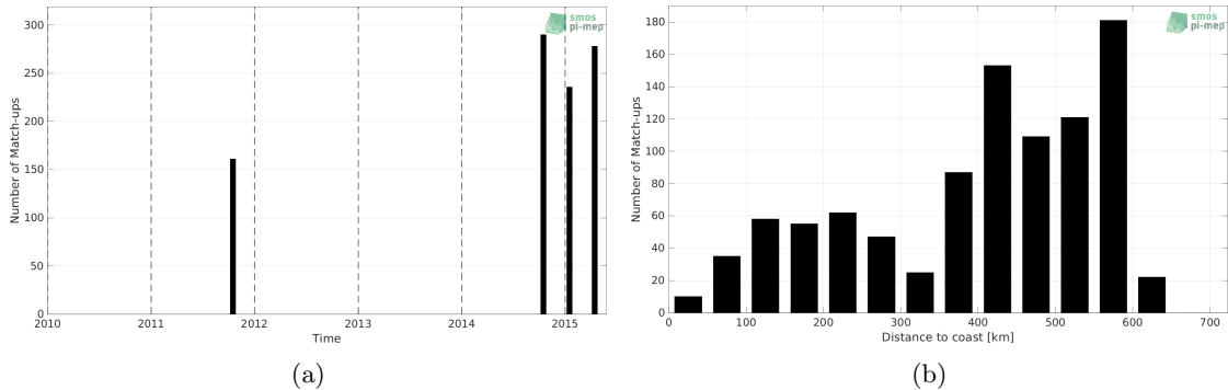
Figure 1: Number of match-ups between TSG (LEGOS-DM) and Aquarius SSS L3 OR v5 - Monthly - Rain mask (NASA-GSFC) SSS as a function of time (a) and as function of the distance to coast (b) over the Bay of Bengal Pi-MEP region and for the full satellite product period.
