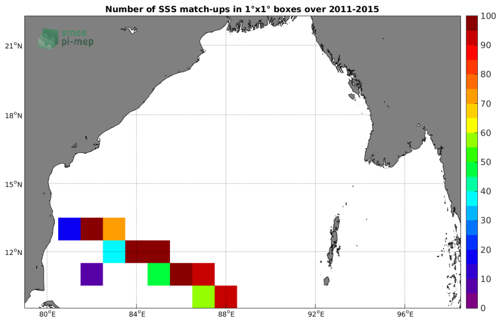
Figure 4: Number of SSS match-ups between TSG-LEGOS-DM SSS and the Aquarius-L3-OR-V5-MONTHLY-RAIN-MASK-1DEG SSS product for the Bay of Bengal Pi-MEP region over 1°x1° boxes and for the full satellite product period.
