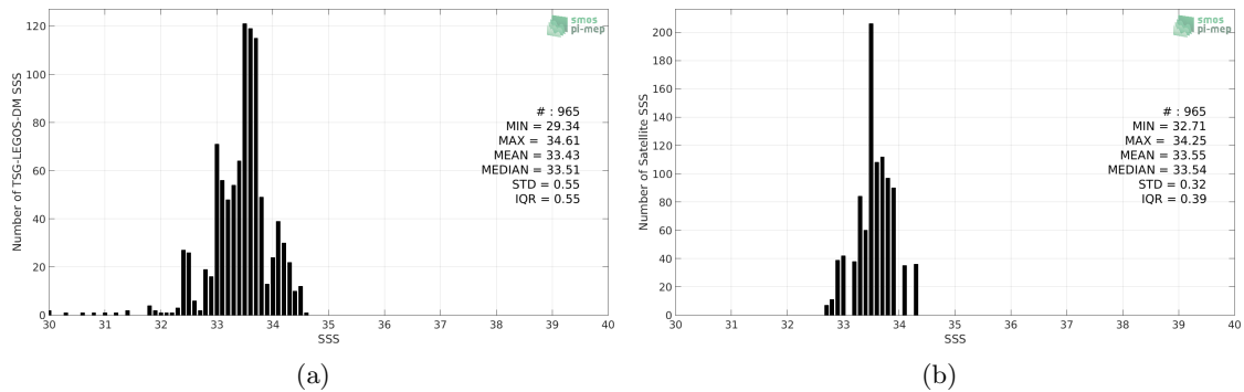
Figure 2: Histograms of SSS from TSG-LEGOS-DM (a) and Aquarius-L3-OR-V5-MONTHLY-RAIN-MASK-1DEG (b) considering all match-up pairs per bins of 0.1 over the Bay of Bengal Pi-MEP region and for the full satellite product period.
