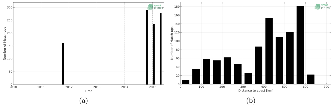
Figure 1: Number of match-ups between TSG-LEGOS-DM and Aquarius-L3-OR-V5-MONTHLY-RAIN-MASK-1DEG SSS as a function of time (a) and as function of the distance to coast (b) over the Bay of Bengal Pi-MEP region and for the full satellite product period.
