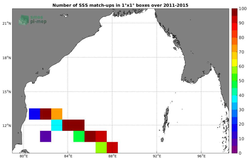
Figure 4: Number of SSS match-ups between TSG-LEGOS-DM SSS and the Aquarius-L3-OR-V5-MONTHLY-RAIN-MASK-1DEG SSS product for the Bay of Bengal Pi-MEP region over 1^\circ \times 1^\circ boxes and for the full satellite product period.
