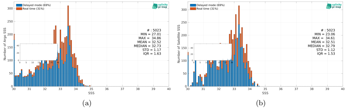
Figure 3: Histograms of SSS from Argo (a) and Aquarius SSS L3 OR v5 - Monthly - Rain mask (NASA-GSFC) (b) considering all match-up pairs per bins of 0.1 over the Bay of Bengal Pi-MEP region and for the full satellite product period.
