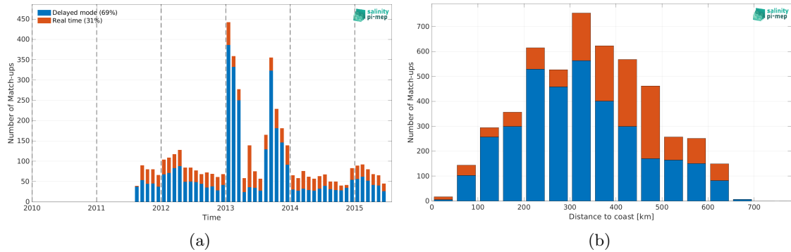
Figure 2: Number of match-ups between Argo and Aquarius SSS L3 OR v5 - Monthly - Rain mask (NASA-GSFC) SSS as a function of time (a) and as function of the distance to coast (b) over the Bay of Bengal Pi-MEP region and for the full satellite product period.
