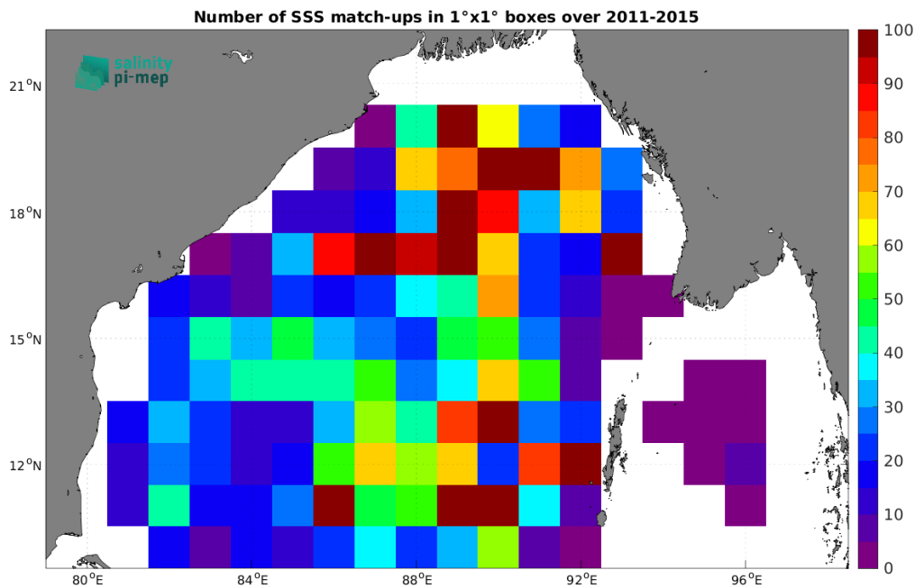
Figure 5: Number of SSS match-ups between Argo SSS and the Aquarius SSS L3 OR v5 - Monthly - Rain mask (NASA-GSFC) SSS product for the Bay of Bengal Pi-MEP region over 1^\circ \times 1^\circ boxes and for the full satellite product period.
