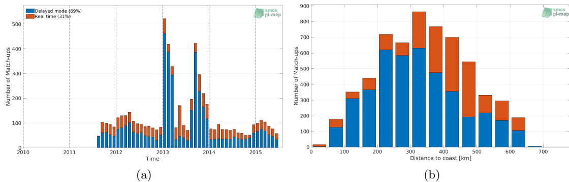
Figure 1: Number of match-ups between Argo and Aquarius SSS L3 OR v5 - Monthly - Rain mask (NASA-GSFC) SSS as a function of time (a) and as function of the distance to coast (b) over the Bay of Bengal Pi-MEP region and for the full satellite product period.
