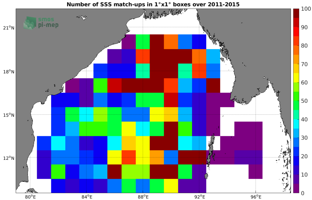
Figure 4: Number of SSS match-ups between Argo SSS and the Aquarius SSS L3 OR v5 - Monthly - Rain mask (NASA-GSFC) SSS product for the Bay of Bengal Pi-MEP region over 1^\circ \times 1^\circ boxes and for the full satellite product period.
