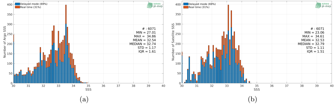
Figure 2: Histograms of SSS from Argo (a) and Aquarius SSS L3 OR v5 - Monthly - Rain mask (NASA-GSFC) (b) considering all match-up pairs per bins of 0.1 over the Bay of Bengal Pi-MEP region and for the full satellite product period.
