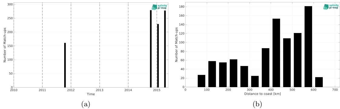
Figure 1: Number of match-ups between TSG (LEGOS-DM) and Aquarius SSS L3 CAP v5 - 7-Day running (JPL) SSS as a function of time (a) and as function of the distance to coast (b) over the Bay of Bengal Pi-MEP region and for the full satellite product period.
