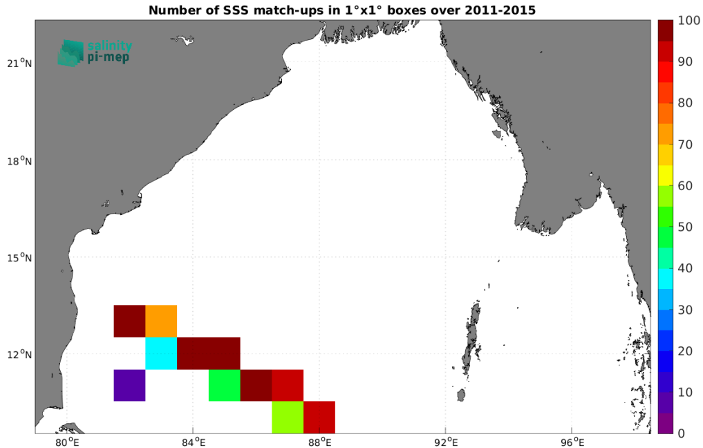
Figure 4: Number of SSS match-ups between TSG (LEGOS-DM) SSS and the Aquarius SSS L3 CAP v5 - 7-Day running (JPL) SSS product for the Bay of Bengal Pi-MEP region over 1^\circ \times 1^\circ boxes and for the full satellite product period.
