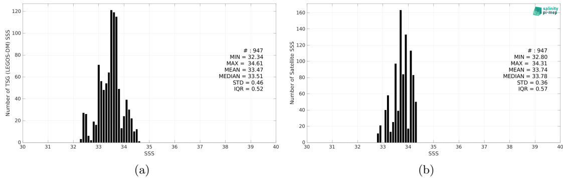
Figure 2: Histograms of SSS from TSG (LEGOS-DM) (a) and Aquarius SSS L3 CAP v5 - 7-Day running (JPL) (b) considering all match-up pairs per bins of 0.1 over the Bay of Bengal Pi-MEP region and for the full satellite product period.
