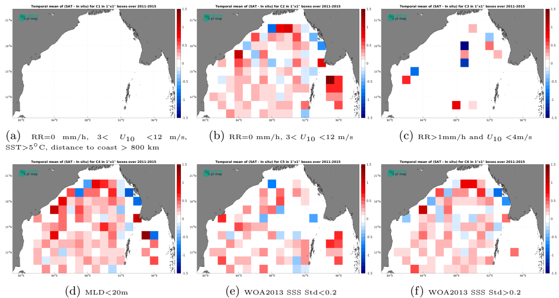
Figure 14: Temporal mean gridded over spatial boxes of size 1^\circ \times 1^\circ of \Delta SSS (Aquarius SSS L3 CAP v5 - 7-Day running (JPL) - Argo) for 6 different subdatasets corresponding to:RR=0 mm/h, 3 < U_{10} < 12 m/s, SST >5^\circ C, distance to coast > 800 km (a), RR=0 mm/h, 3 < U_{10} < 12 m/s (b), RR >1 mm/h and U_{10} < 4 m/s (c),MLD <20 m (d),WOA2013 SSS Std <0.2 (e),WOA2013 SSS Std >0.2 (f).
