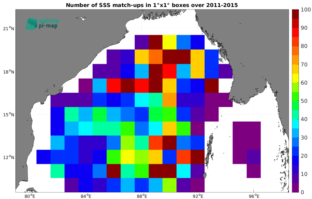
Figure 5: Number of SSS match-ups between Argo SSS and the Aquarius SSS L3 CAP v5 - 7-Day running (JPL) SSS product for the Bay of Bengal Pi-MEP region over 1^\circ \times 1^\circ boxes and for the full satellite product period.
