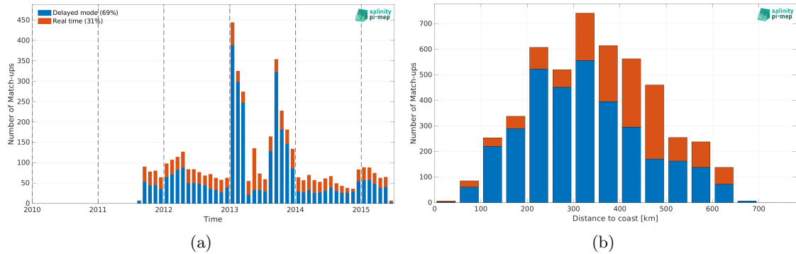
Figure 2: Number of match-ups between Argo and Aquarius SSS L3 CAP v5 - 7-Day running (JPL) SSS as a function of time (a) and as function of the distance to coast (b) over the Bay of Bengal Pi-MEP region and for the full satellite product period.
