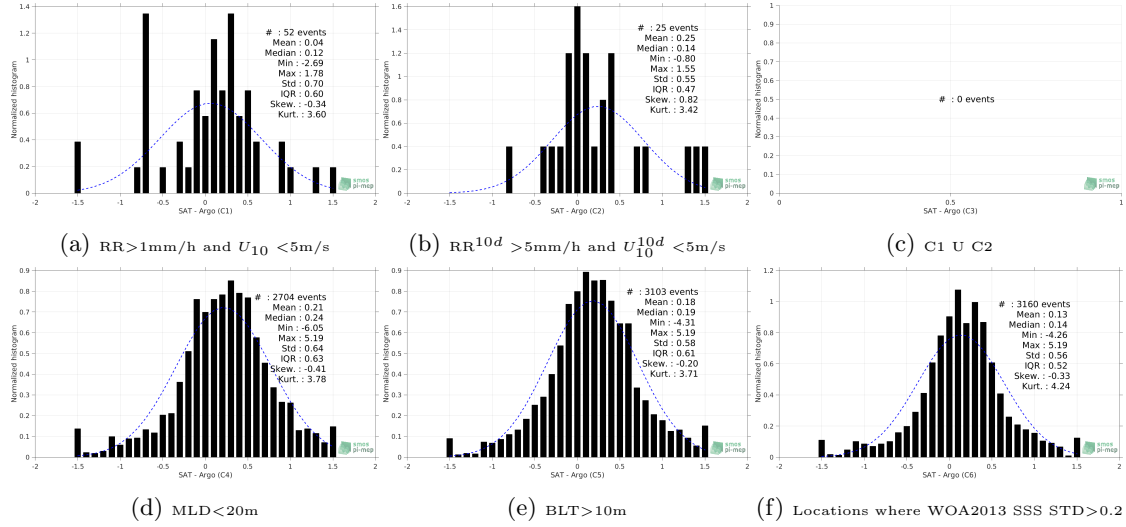
Figure 13: Normalized histogram of \Delta SSS (Aquarius-L3-JPL-V5-7DAY-RUNNING - Argo) for 6 different subdatasets corresponding to: RR > 1mm/h and U_{10} < 5\text{m/s} (a), RR^{10d} > 5\text{mm/h} and U_{10}^{10d} < 5\text{m/s} (b), C1 U C2 (c), MLD < 20m (d), BLT > 10m (e), Locations where WOA2013 SSS STD > 0.2 (f).
