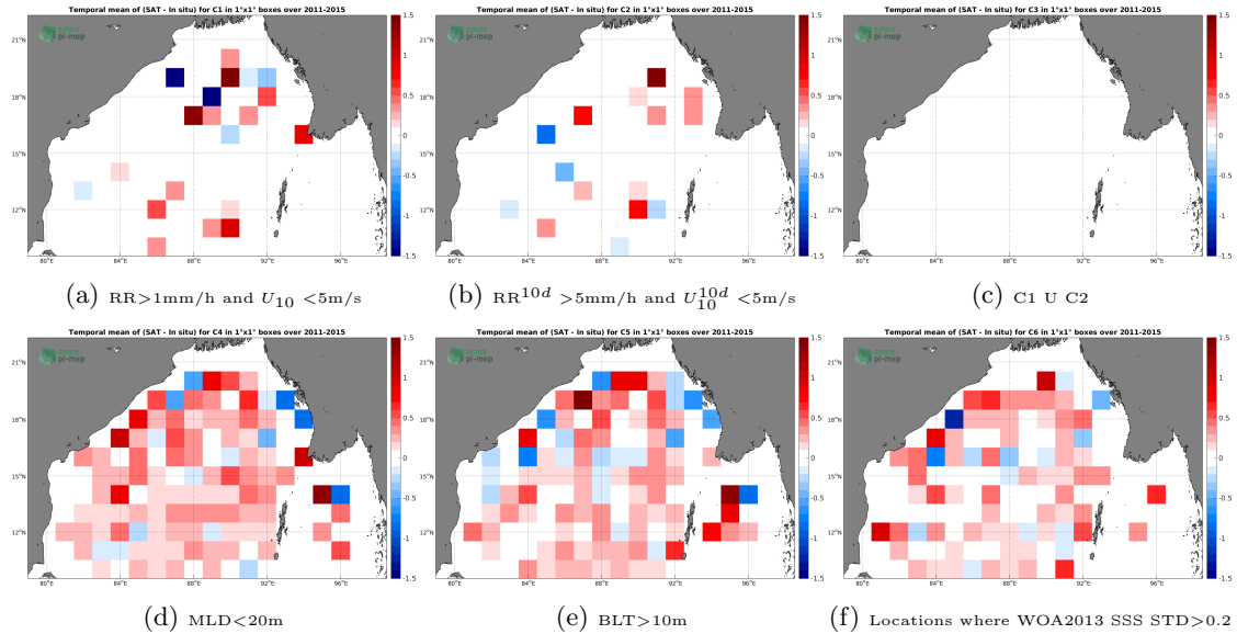
Figure 12: Temporal mean gridded over spatial boxes of size 1^\circ \times 1^\circ of \Delta\text{SSS} (Aquarius-L3-JPL-V5-7DAY-RUNNING - Argo) for 6 different subdatasets corresponding to: \text{RR} > 1\text{mm/h} and U_{10} < 5\text{m/s} (a), \text{RR}^{10d} > 5\text{mm/h} and U_{10}^{10d} < 5\text{m/s} (b), C1 U C2 (c), \text{MLD} < 20\text{m} (d), \text{BLT} > 10\text{m} (e), Locations where WOA2013 SSS STD > 0.2 (f).
