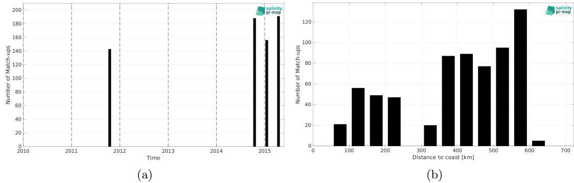
Figure 2: Number of match-ups between TSG (LEGOS-DM) and Aquarius SSS L3 CAP v5 - Monthly (JPL) SSS as a function of time (a) and as function of the distance to coast (b) over the Bay of Bengal Pi-MEP region and for the full satellite product period.
