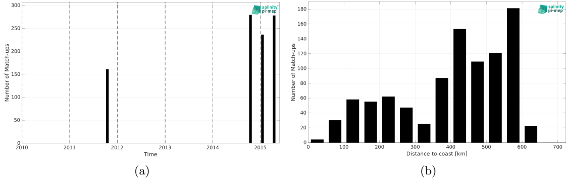
Figure 1: Number of match-ups between TSG (LEGOS-DM) and Aquarius SSS L3 CAP v5 - Monthly (JPL) SSS as a function of time (a) and as function of the distance to coast (b) over the Bay of Bengal Pi-MEP region and for the full satellite product period.
