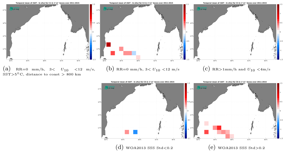
Figure 12: Temporal mean gridded over spatial boxes of size 1^\circ \times 1^\circ of \Delta\text{SSS} (Aquarius SSS L3 CAP v5 - Monthly (JPL) - TSG (LEGOS-DM)) for 5 different subdatasets corresponding to:RR=0 mm/h, 3 < U_{10} < 12 m/s, SST >5^\circ\text{C} , distance to coast > 800 km (a), RR=0 mm/h, 3 < U_{10} < 12 m/s (b), RR >1 mm/h and U_{10} < 4 m/s (c), WOA2013 SSS Std <0.2 (d), WOA2013 SSS Std >0.2 (e).
