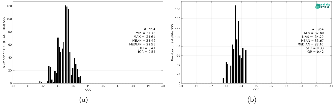
Figure 2: Histograms of SSS from TSG (LEGOS-DM) (a) and Aquarius SSS L3 CAP v5 - Monthly (JPL) (b) considering all match-up pairs per bins of 0.1 over the Bay of Bengal Pi-MEP region and for the full satellite product period.
