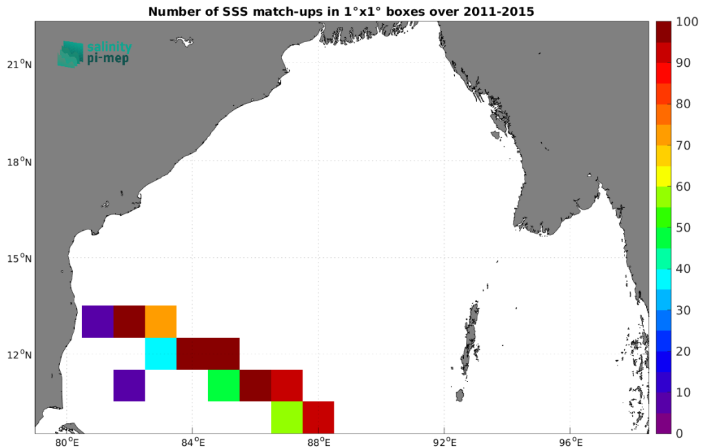
Figure 4: Number of SSS match-ups between TSG (LEGOS-DM) SSS and the Aquarius SSS L3 CAP v5 - Monthly (JPL) SSS product for the Bay of Bengal Pi-MEP region over 1^\circ \times 1^\circ boxes and for the full satellite product period.
