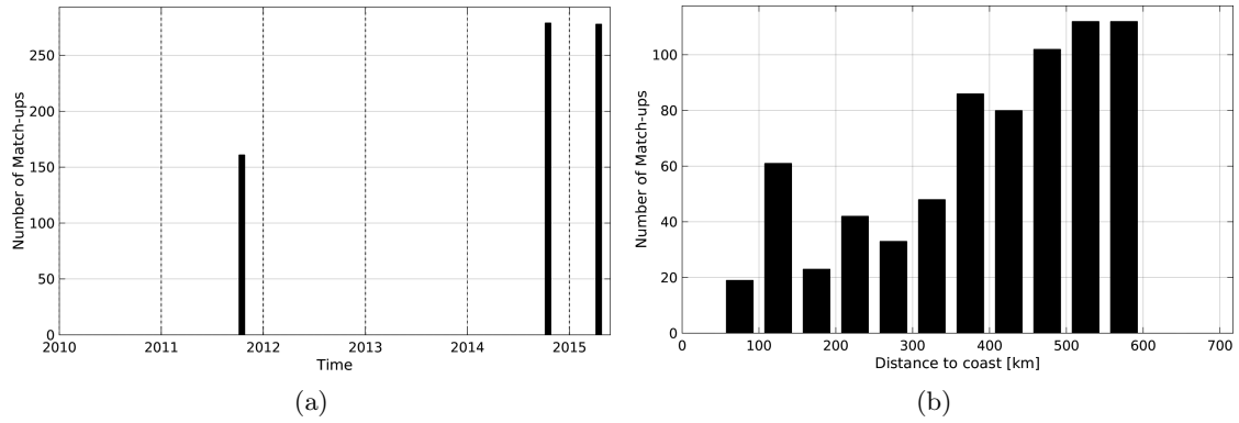
Figure 1: Number of match-ups between TSG-LEGOS-DM and Aquarius-L3-JPL-V4-MONTHLY SSS as a function of time (a) and as function of the distance to coast (b) over the Bay of Bengal Pi-MEP region and for the full satellite product period.
