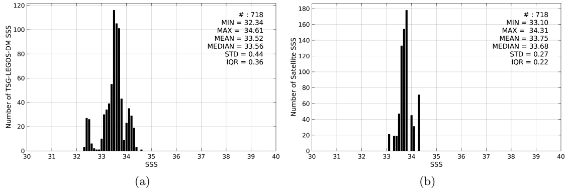
Figure 2: Histograms of SSS from TSG-LEGOS-DM (a) and Aquarius-L3-JPL-V4-MONTHLY (b) considering all match-up pairs per bins of 0.1 over the Bay of Bengal Pi-MEP region and for the full satellite product period.
