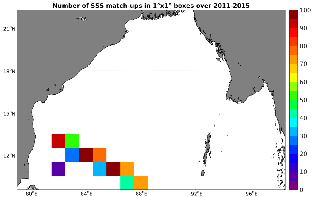
Figure 4: Number of SSS match-ups between TSG-LEGOS-DM SSS and the Aquarius-L3-JPL-V4-MONTHLY SSS product for the Bay of Bengal Pi-MEP region over 1°x1° boxes and for the full satellite product period.
