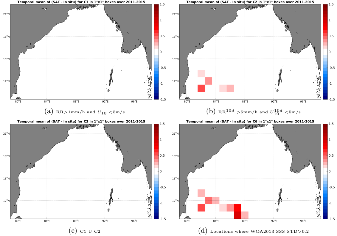
Figure 12: Temporal mean gridded over spatial boxes of size 1^\circ \times 1^\circ of \Delta SSS (Aquarius-L3-JPL-V4-MONTHLY - TSG-LEGOS-DM) for 4 different subdatasets corresponding to: RR > 1mm/h and U_{10} < 5 m/s (a), RR^{10d} > 5 mm/h and U_{10}^{10d} < 5 m/s (b), C1 U C2 (c), Locations where WOA2013 SSS STD > 0.2 (d).
