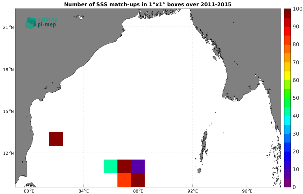
Figure 5: Number of SSS match-ups between TSG (LEGOS-DM) SSS and the Aquarius SSS L2 OR v5 (NASA-GSFC) SSS product for the Bay of Bengal Pi-MEP region over 1^\circ \times 1^\circ boxes and for the full satellite product period.
