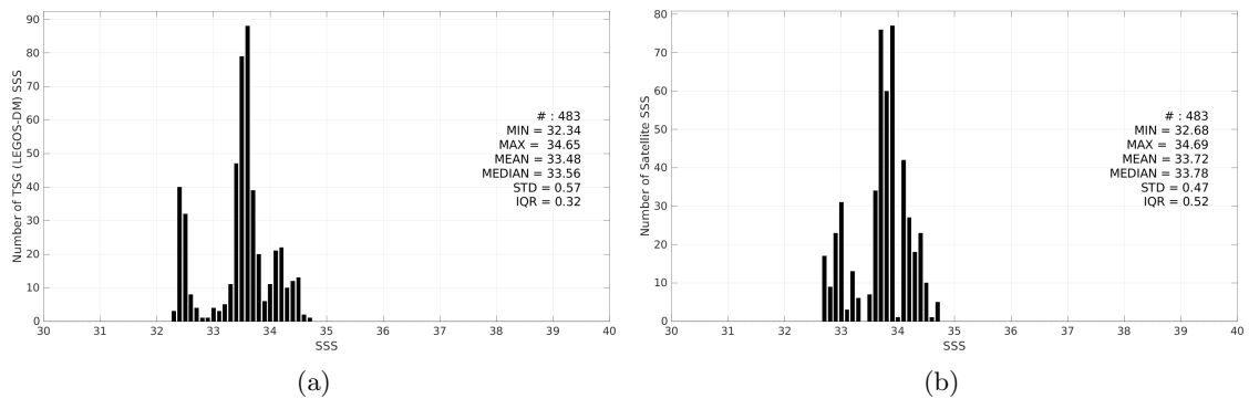
Figure 3: Histograms of SSS from TSG (LEGOS-DM) (a) and Aquarius SSS L2 OR v5 (NASA-GSFC) (b) considering all match-up pairs per bins of 0.1 over the Bay of Bengal Pi-MEP region and for the full satellite product period.
