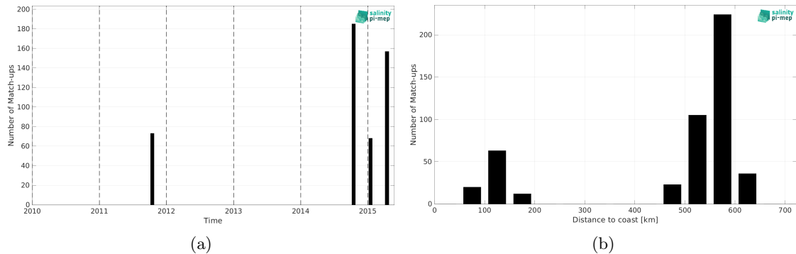
Figure 2: Number of match-ups between TSG (LEGOS-DM) and Aquarius SSS L2 OR v5 (NASA-GSFC) SSS as a function of time (a) and as function of the distance to coast (b) over the Bay of Bengal Pi-MEP region and for the full satellite product period.
