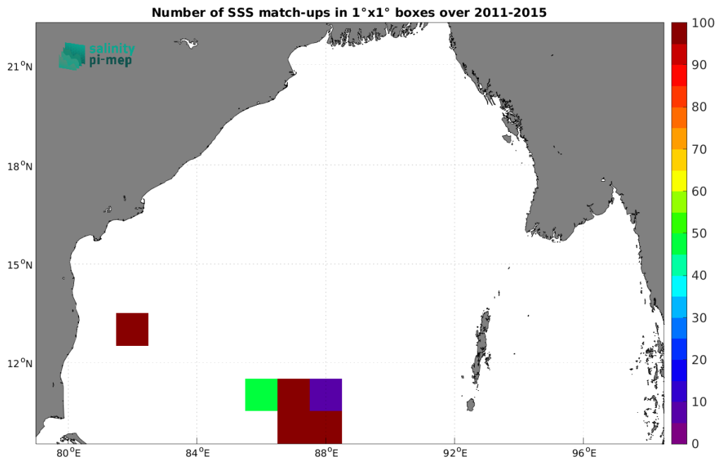
Figure 4: Number of SSS match-ups between TSG (LEGOS-DM) SSS and the Aquarius SSS L2 OR v5 (NASA-GSFC) SSS product for the Bay of Bengal Pi-MEP region over 1^\circ \times 1^\circ boxes and for the full satellite product period.
