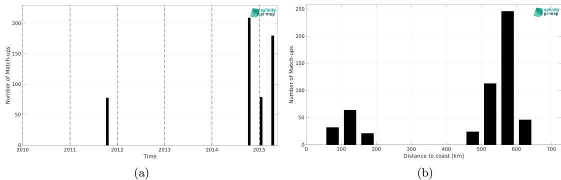
Figure 1: Number of match-ups between TSG (LEGOS-DM) and Aquarius SSS L2 OR v5 (NASA-GSFC) SSS as a function of time (a) and as function of the distance to coast (b) over the Bay of Bengal Pi-MEP region and for the full satellite product period.
