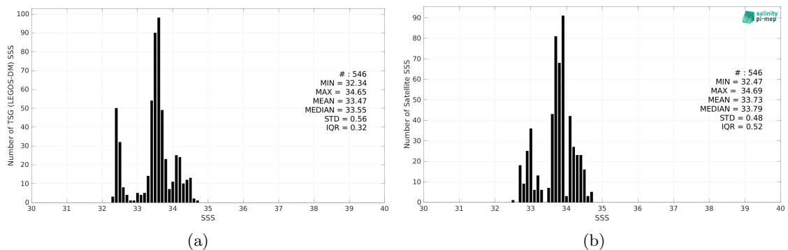
Figure 2: Histograms of SSS from TSG (LEGOS-DM) (a) and Aquarius SSS L2 OR v5 (NASA-GSFC) (b) considering all match-up pairs per bins of 0.1 over the Bay of Bengal Pi-MEP region and for the full satellite product period.
