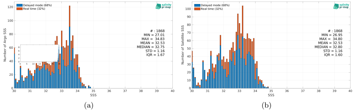
Figure 2: Histograms of SSS from Argo (a) and Aquarius SSS L2 OR v5 (NASA-GSFC) (b) considering all match-up pairs per bins of 0.1 over the Bay of Bengal Pi-MEP region and for the full satellite product period.
