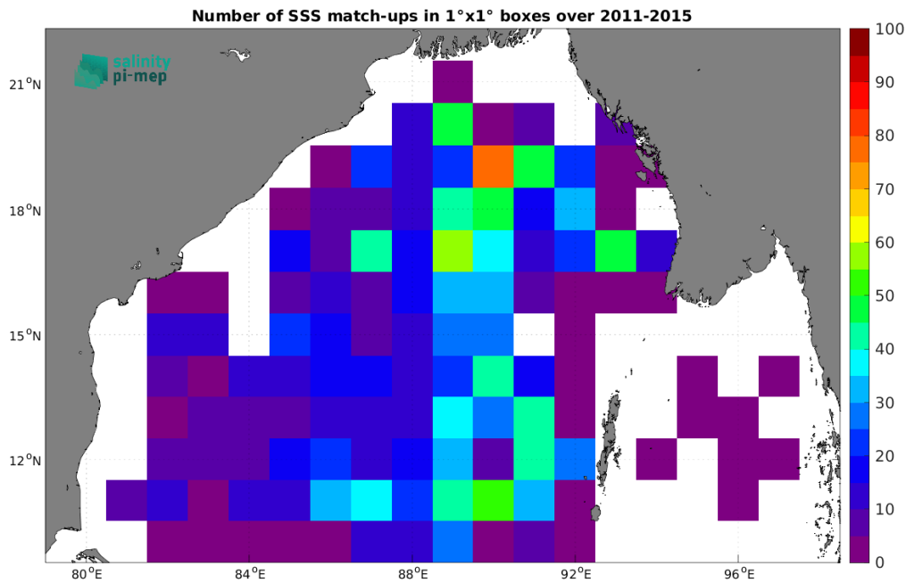
Figure 4: Number of SSS match-ups between Argo SSS and the Aquarius SSS L2 OR v5 (NASA-GSFC) SSS product for the Bay of Bengal Pi-MEP region over 1^\circ \times 1^\circ boxes and for the full satellite product period.
