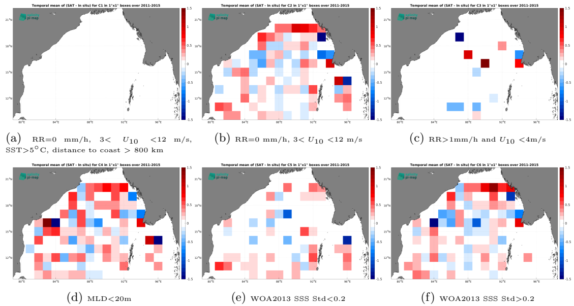
Figure 12: Temporal mean gridded over spatial boxes of size 1^\circ \times 1^\circ of \Delta SSS (Aquarius SSS L2 OR v5 (NASA-GSFC) - Argo) for 6 different subdatasets corresponding to:RR=0 mm/h, 3 < U_{10} < 12 m/s, SST > 5^\circ\text{C} , distance to coast > 800 km (a), RR=0 mm/h, 3 < U_{10} < 12 m/s (b), RR > 1 mm/h and U_{10} < 4 m/s (c),MLD < 20 m (d),WOA2013 SSS Std < 0.2 (e),WOA2013 SSS Std > 0.2 (f).
