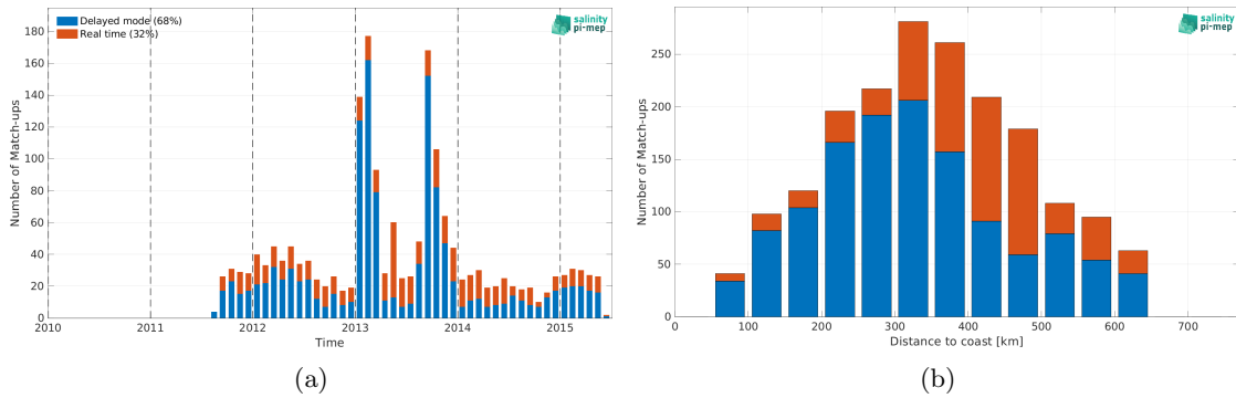
Figure 1: Number of match-ups between Argo and Aquarius SSS L2 OR v5 (NASA-GSFC) SSS as a function of time (a) and as function of the distance to coast (b) over the Bay of Bengal Pi-MEP region and for the full satellite product period.
