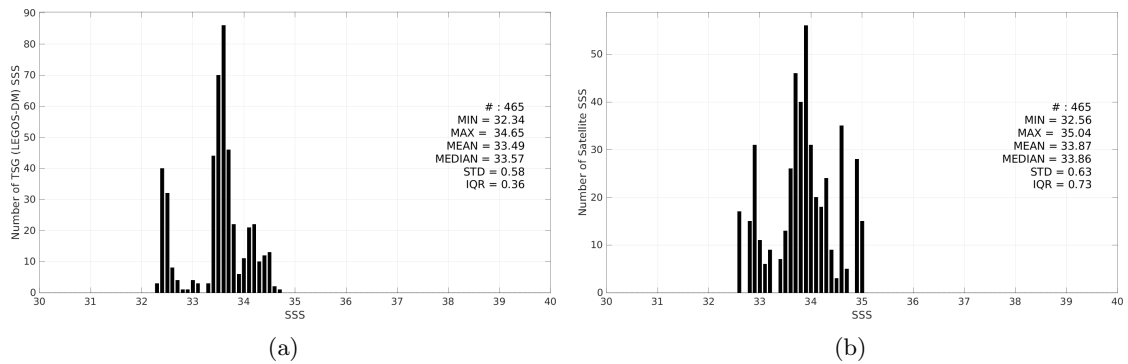
Figure 3: Histograms of SSS from TSG (LEGOS-DM) (a) and Aquarius SSS L2 CAP v5 (JPL) (b) considering all match-up pairs per bins of 0.1 over the Bay of Bengal Pi-MEP region and for the full satellite product period.
