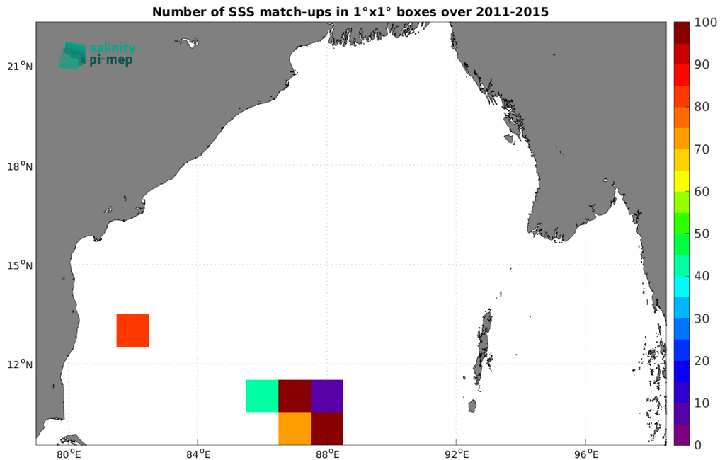
Figure 5: Number of SSS match-ups between TSG (LEGOS-DM) SSS and the Aquarius SSS L2 CAP v5 (JPL) SSS product for the Bay of Bengal Pi-MEP region over 1^\circ \times 1^\circ boxes and for the full satellite product period.
