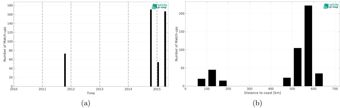
Figure 2: Number of match-ups between TSG (LEGOS-DM) and Aquarius SSS L2 CAP v5 (JPL) SSS as a function of time (a) and as function of the distance to coast (b) over the Bay of Bengal Pi-MEP region and for the full satellite product period.
