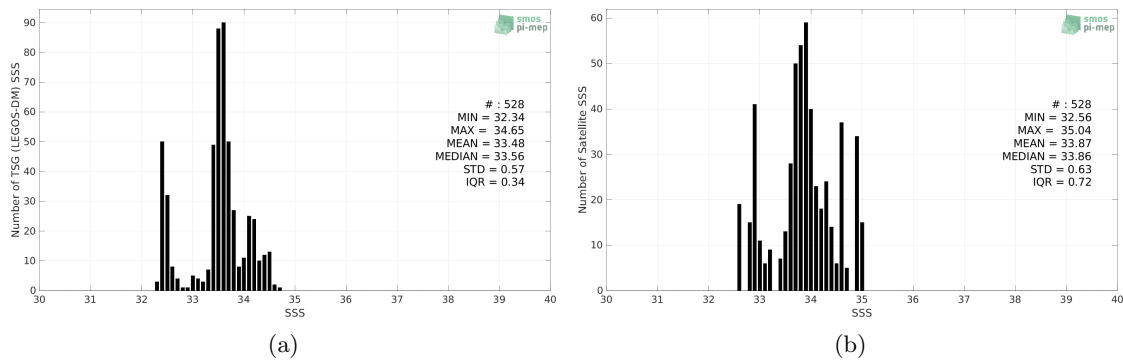
Figure 2: Histograms of SSS from TSG (LEGOS-DM) (a) and Aquarius SSS L2 CAP v5 (JPL) (b) considering all match-up pairs per bins of 0.1 over the Bay of Bengal Pi-MEP region and for the full satellite product period.
