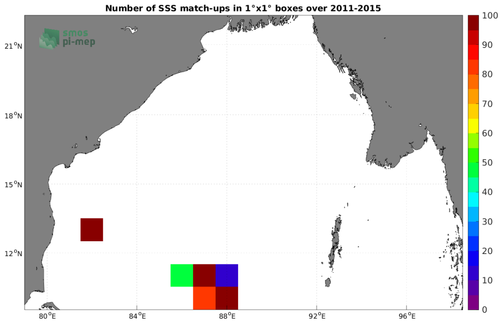
Figure 4: Number of SSS match-ups between TSG (LEGOS-DM) SSS and the Aquarius SSS L2 CAP v5 (JPL) SSS product for the Bay of Bengal Pi-MEP region over 1^\circ \times 1^\circ boxes and for the full satellite product period.
