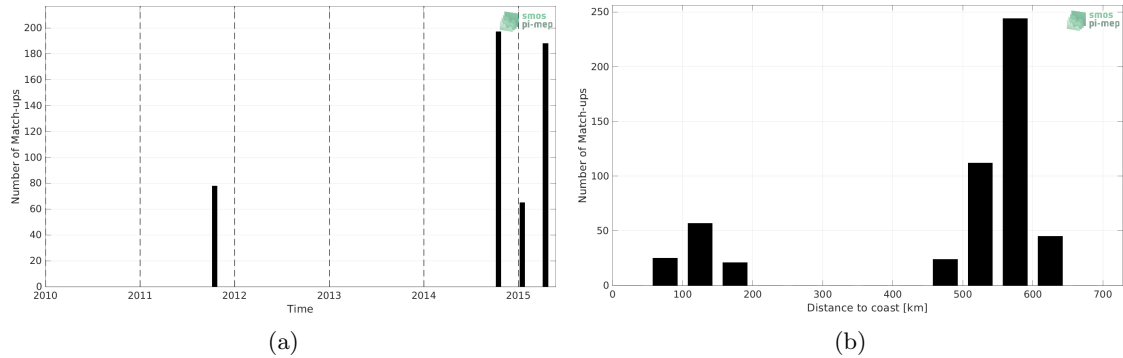
Figure 1: Number of match-ups between TSG (LEGOS-DM) and Aquarius SSS L2 CAP v5 (JPL) SSS as a function of time (a) and as function of the distance to coast (b) over the Bay of Bengal Pi-MEP region and for the full satellite product period.
