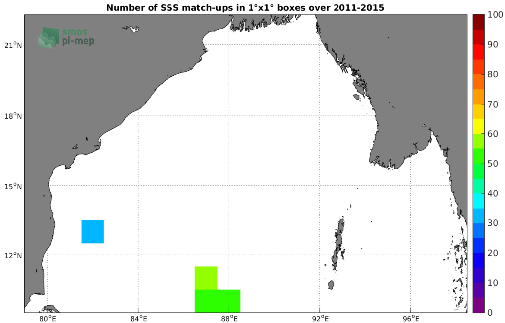
Figure 4: Number of SSS match-ups between TSG-LEGOS-DM SSS and the Aquarius-L2-JPL-V5 SSS product for the Bay of Bengal Pi-MEP region over 1^\circ \times 1^\circ boxes and for the full satellite product period.
