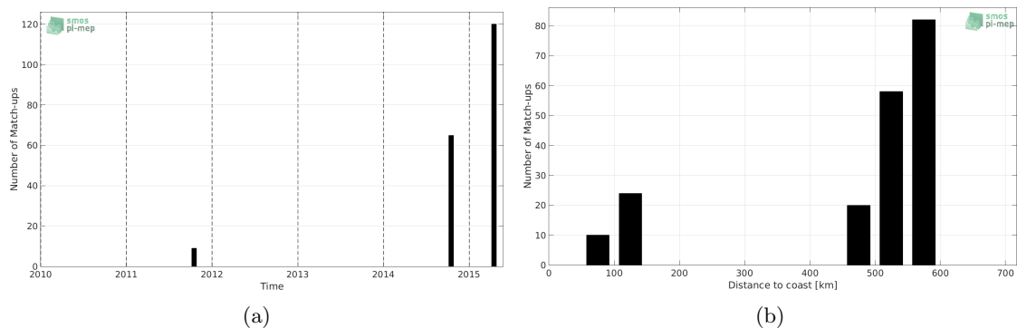
Figure 1: Number of match-ups between TSG-LEGOS-DM and Aquarius-L2-JPL-V5 SSS as a function of time (a) and as function of the distance to coast (b) over the Bay of Bengal Pi-MEP region and for the full satellite product period.
