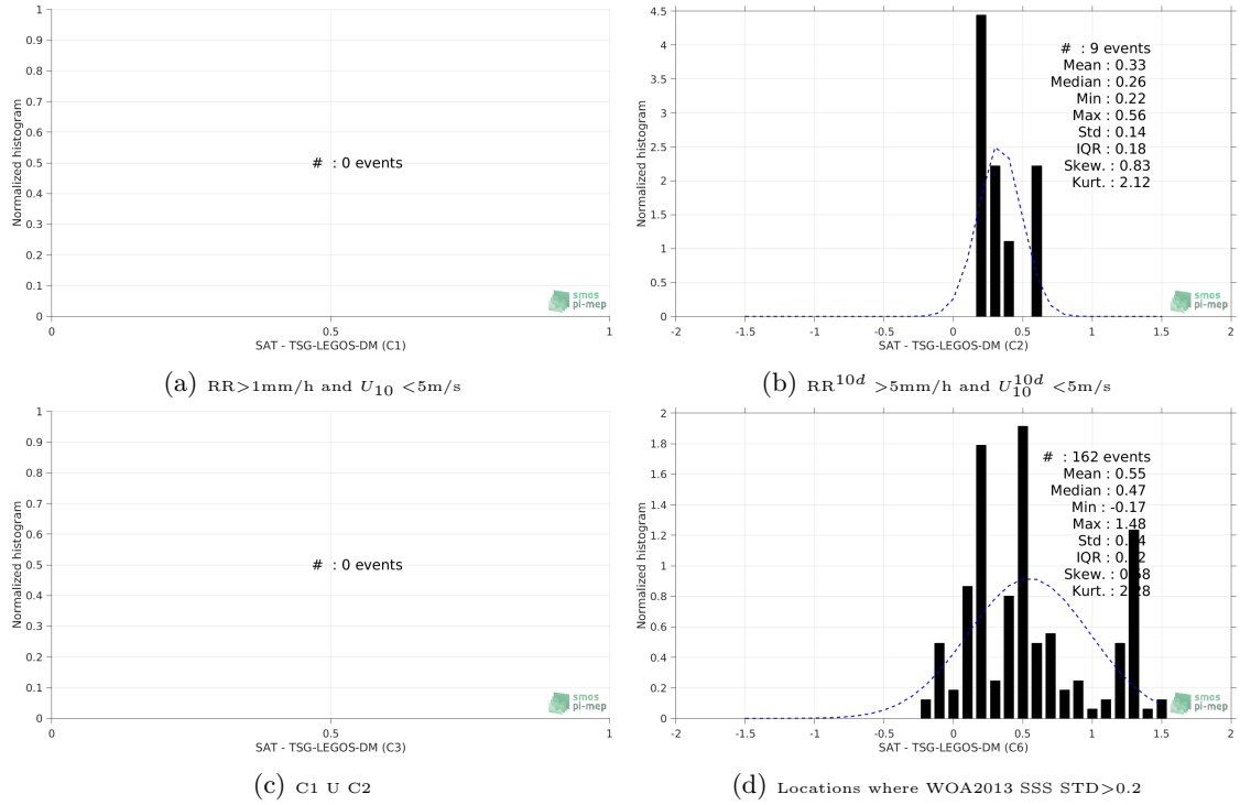
Figure 13: Normalized histogram of \Delta\text{SSS} (Aquarius-L2-JPL-V5 - TSG-LEGOS-DM) for 6 different subdatasets corresponding to: RR > 1\text{mm/h} and U_{10} < 5\text{m/s} (a), RR^{10d} > 5\text{mm/h} and U_{10}^{10d} < 5\text{m/s} (b), C1 \cup C2 (c), Locations where WOA2013 SSS STD > 0.2 (d).
