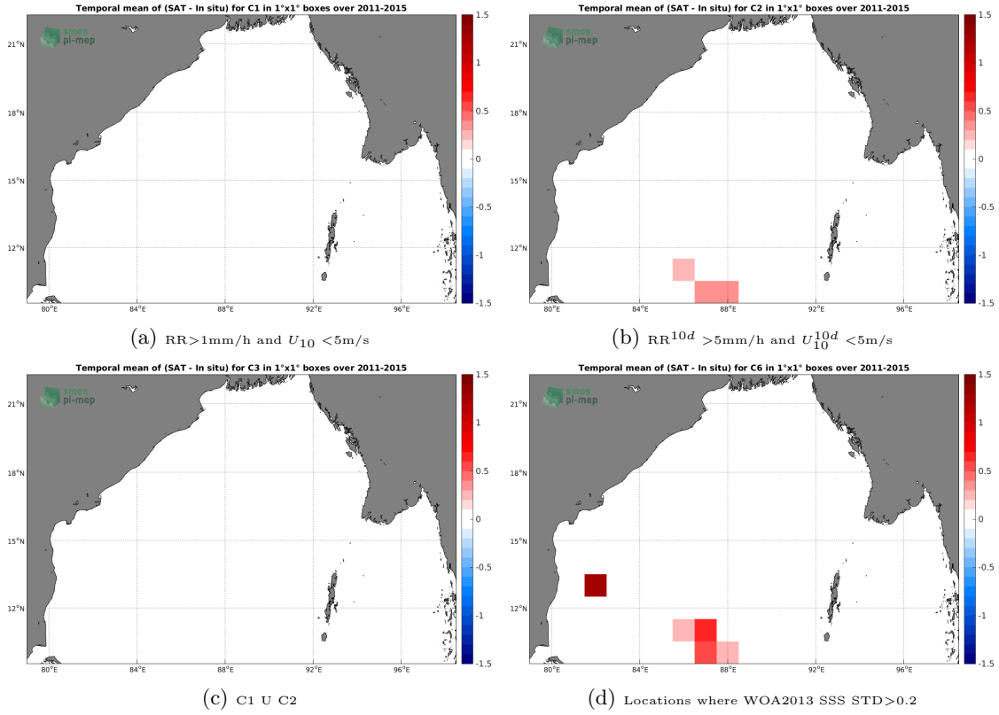
Figure 12: Temporal mean gridded over spatial boxes of size 1^\circ \times 1^\circ of \Delta SSS (Aquarius-L2-JPL-V5 - TSG-LEGOS-DM) for 4 different subdatasets corresponding to: RR > 1mm/h and U_{10} < 5m/s (a), RR^{10d} > 5mm/h and U_{10}^{10d} < 5m/s (b), C1 U C2 (c), Locations where WOA2013 SSS STD > 0.2 (d).
