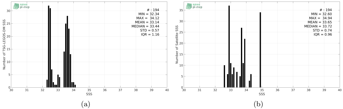
Figure 2: Histograms of SSS from TSG-LEGOS-DM (a) and Aquarius-L2-JPL-V5 (b) considering all match-up pairs per bins of 0.1 over the Bay of Bengal Pi-MEP region and for the full satellite product period.
