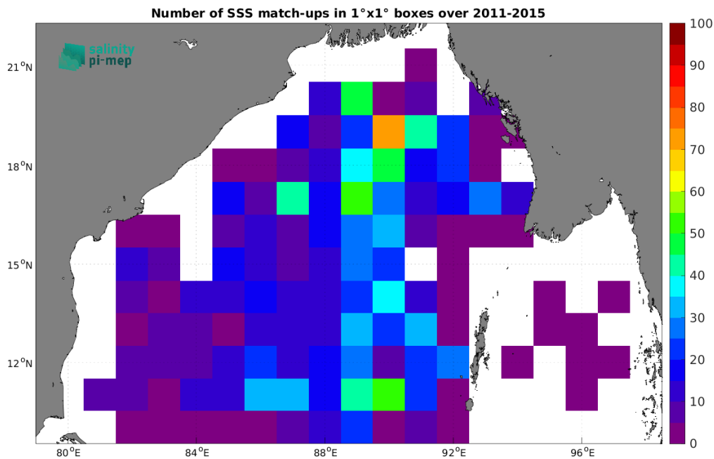
Figure 5: Number of SSS match-ups between Argo SSS and the Aquarius SSS L2 CAP v5 (JPL) SSS product for the Bay of Bengal Pi-MEP region over 1^\circ \times 1^\circ boxes and for the full satellite product period.
