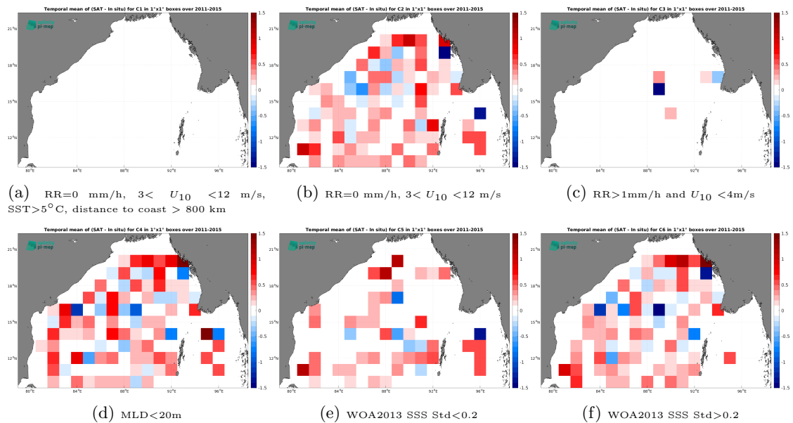
Figure 14: Temporal mean gridded over spatial boxes of size 1^\circ \times 1^\circ of \Delta SSS (Aquarius SSS L2 CAP v5 (JPL) - Argo) for 6 different subdatasets corresponding to:RR=0 mm/h, 3 < U_{10} < 12 m/s, SST > 5^\circ\text{C} , distance to coast > 800 km (a), RR=0 mm/h, 3 < U_{10} < 12 m/s (b), RR > 1 mm/h and U_{10} < 4 m/s (c),MLD < 20 m (d),WOA2013 SSS Std < 0.2 (e),WOA2013 SSS Std > 0.2 (f).
