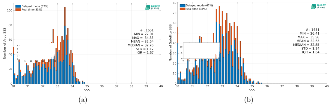
Figure 3: Histograms of SSS from Argo (a) and Aquarius SSS L2 CAP v5 (JPL) (b) considering all match-up pairs per bins of 0.1 over the Bay of Bengal Pi-MEP region and for the full satellite product period.
