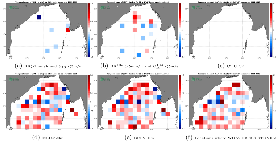
Figure 12: Temporal mean gridded over spatial boxes of size 1^\circ \times 1^\circ of \Delta\text{SSS} (Aquarius-L2-JPL-V5 - Argo) for 6 different subdatasets corresponding to: RR > 1\text{mm/h} and U_{10} < 5\text{m/s} (a), RR^{10d} > 5\text{mm/h} and U_{10}^{10d} < 5\text{m/s} (b), C1 U C2 (c), MLD < 20\text{m} (d), BLT > 10\text{m} (e), Locations where WOA2013 SSS STD > 0.2 (f).
