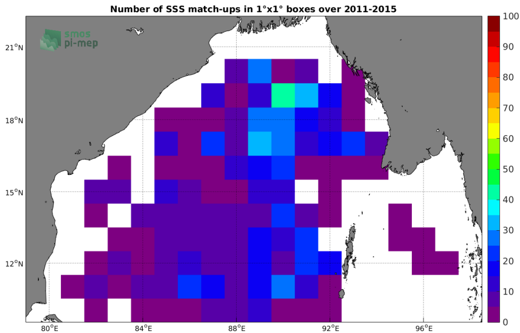
Figure 4: Number of SSS match-ups between Argo SSS and the Aquarius-L2-JPL-V5 SSS product for the Bay of Bengal Pi-MEP region over 1^\circ \times 1^\circ boxes and for the full satellite product period.
