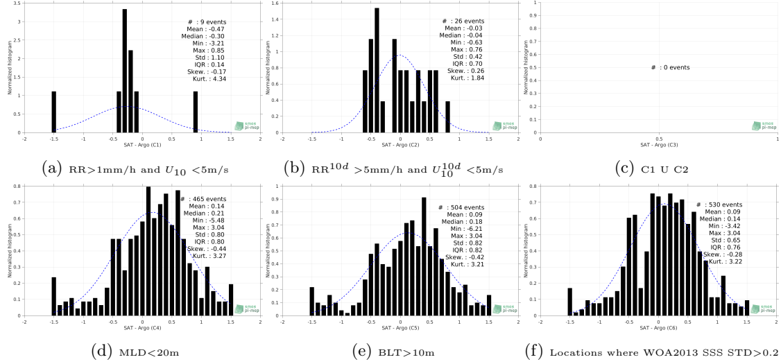
Figure 13: Normalized histogram of \Delta SSS (Aquarius-L2-JPL-V5 - Argo) for 6 different sub-datasets corresponding to: RR > 1\text{mm/h} and U_{10} < 5\text{m/s} (a), RR^{10d} > 5\text{mm/h} and U_{10}^{10d} < 5\text{m/s} (b), C1 U C2 (c), MLD < 20\text{m} (d), BLT > 10\text{m} (e), Locations where WOA2013 SSS STD > 0.2 (f).
