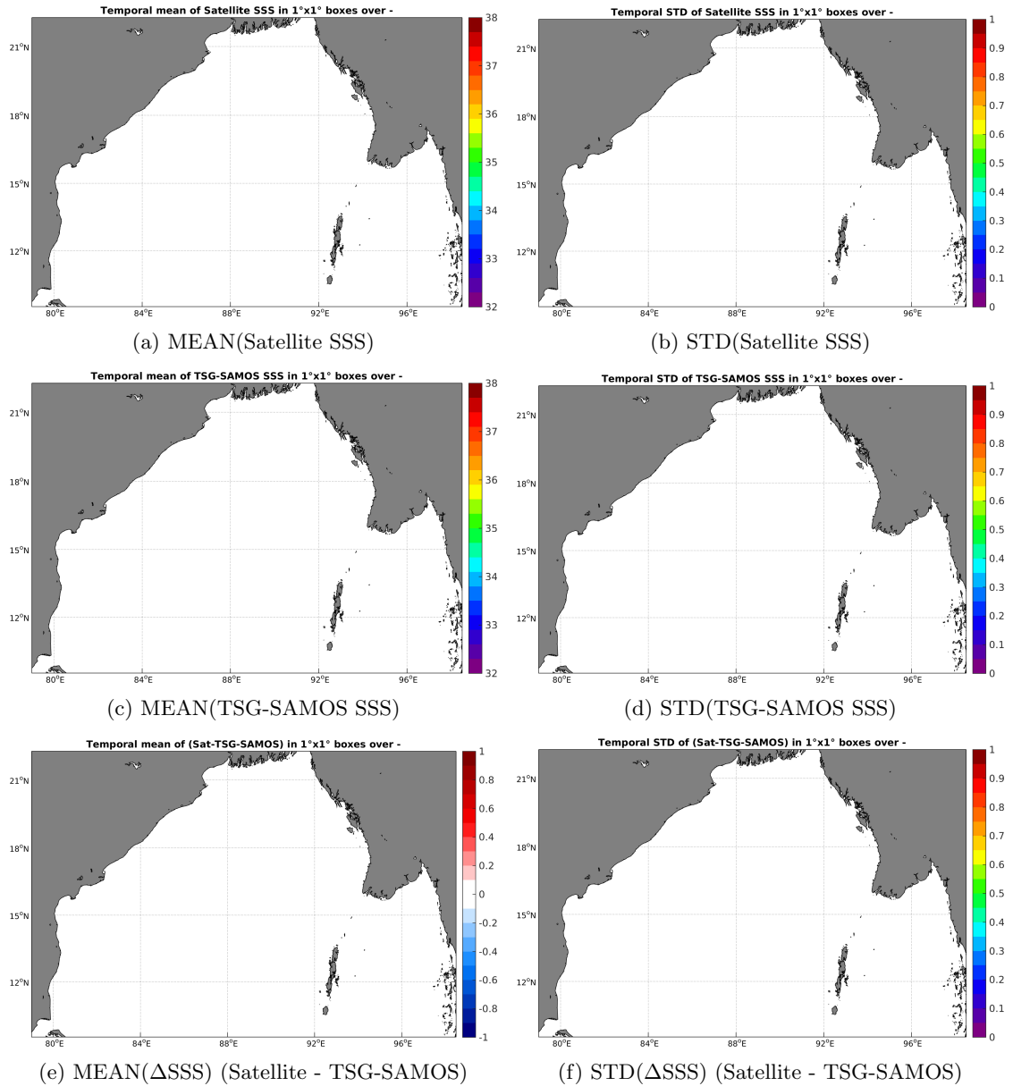
Figure 6: Temporal mean (left) and STD (right) of SSS from AQUARIUS-L2-JPL-V4 (top), TSG-SAMOS (middle), and of \Delta SSS (Satellite - TSG-SAMOS). Only match-up pairs are used to generate these maps.
