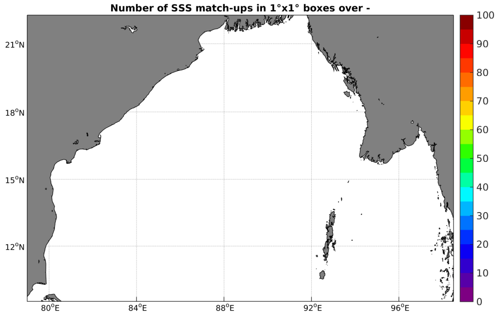
Figure 4: Number of SSS match-ups between TSG-SAMOS SSS and the AQUARIUS-L2-JPL-V4 SSS product for the Bay of Bengal Pi-MEP region over 1^\circ \times 1^\circ boxes and for the full satellite product period.
