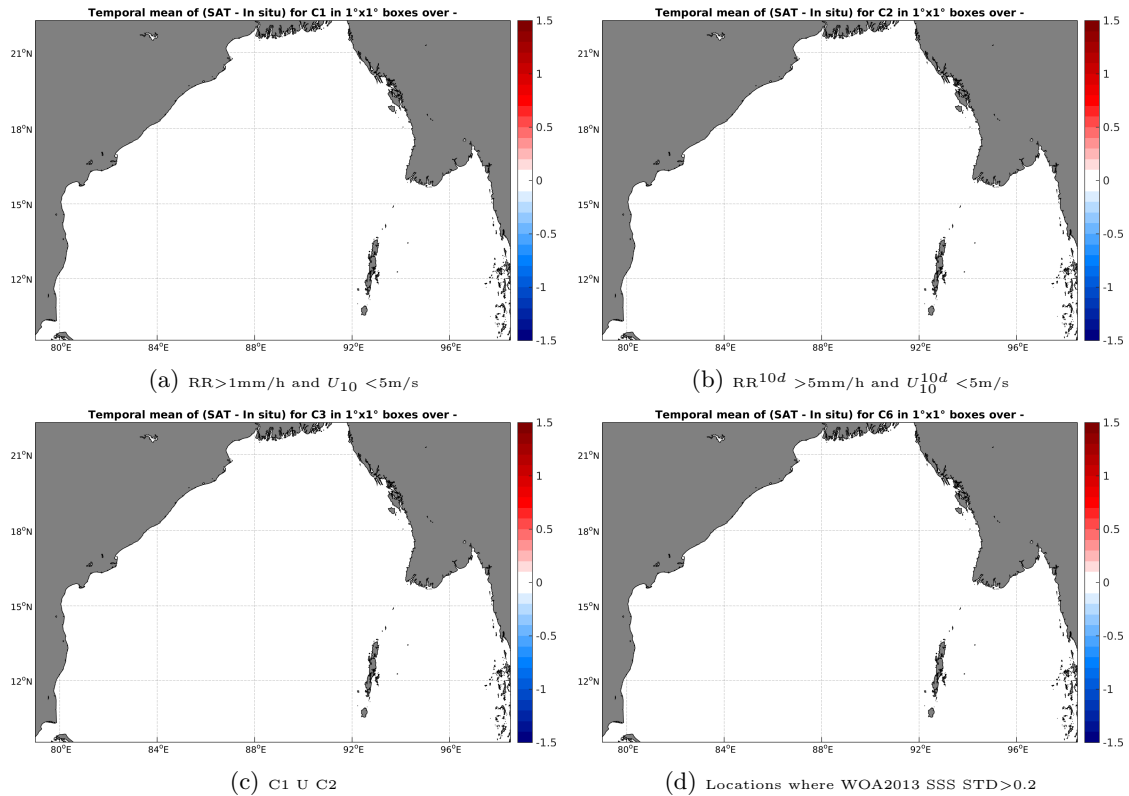
Figure 12: Temporal mean gridded over spatial boxes of size 1^\circ \times 1^\circ of \Delta SSS (AQUARIUS-L2-JPL-V4 - TSG-SAMOS) for 4 different subdatasets corresponding to:RR > 1 mm/h and U_{10} < 5 m/s (a), RR 10d > 5 mm/h and U_{10}^{10d} < 5 m/s (b), C1 U C2 (c),Locations where WOA2013 SSS STD > 0.2 (d).
