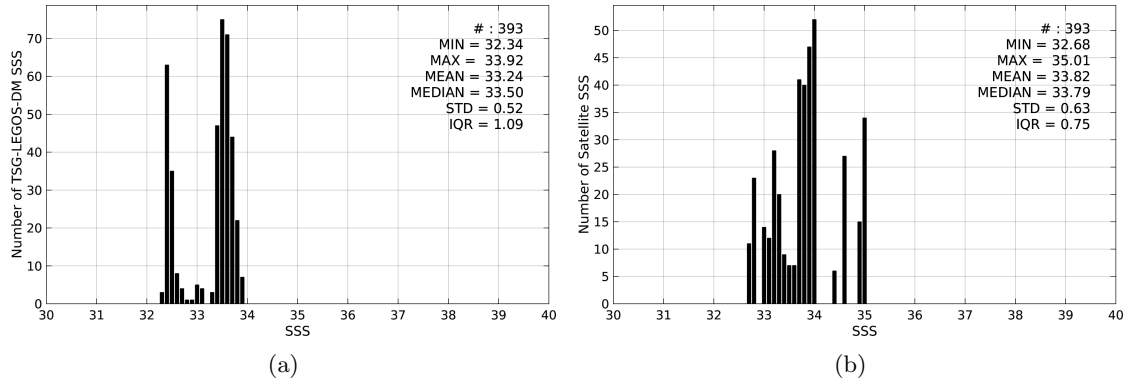
Figure 2: Histograms of SSS from TSG-LEGOS-DM (a) and AQUARIUS-L2-JPL-V4 (b) considering all match-up pairs per bins of 0.1 over the Bay of Bengal Pi-MEP region and for the full satellite product period.
