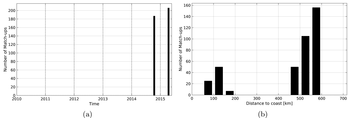
Figure 1: Number of match-ups between TSG-LEGOS-DM and AQUARIUS-L2-JPL-V4 SSS as a function of time (a) and as function of the distance to coast (b) over the Bay of Bengal Pi-MEP region and for the full satellite product period.
