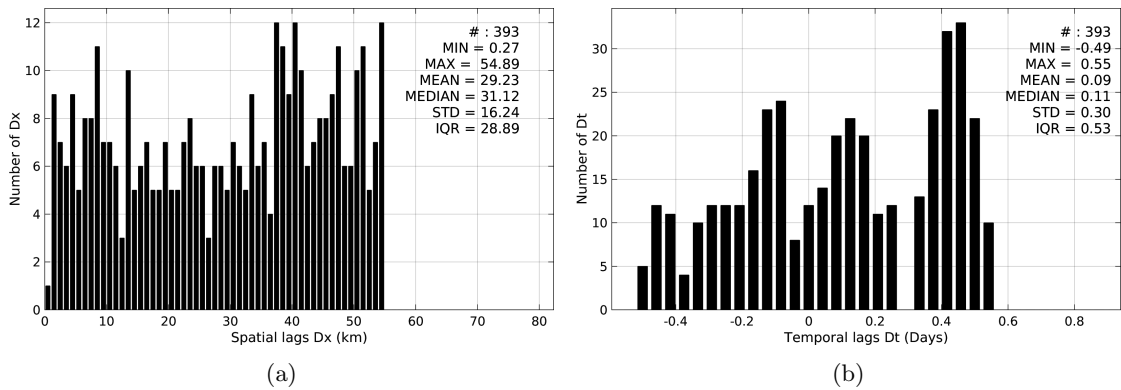
Figure 5: Histograms of the spatial (a) and temporal (b) lags between the time of the TSG-LEGOS-DM measurements and the date of the corresponding AQUARIUS-L2-JPL-V4 SSS product.
