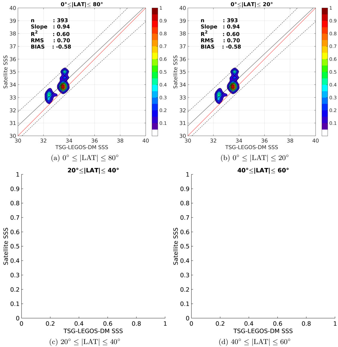
Figure 9: Contour maps of the concentration of AQUARIUS-L2-JPL-V4 SSS (y-axis) versus TSG-LEGOS-DM SSS (x-axis) at match-up pairs for different latitude bands. For each plot, the red line shows x=y . The black thin and dashed lines indicate a linear fit through the data cloud and the \pm 95\% confidence levels, respectively. The number match-up pairs n , the slope and R^2 coefficient of the linear fit, the root mean square (RMS) and the mean bias between satellite and in situ data are indicated for each latitude band in each plots.
