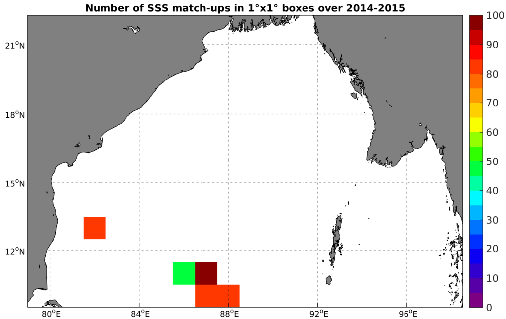
Figure 4: Number of SSS match-ups between TSG-LEGOS-DM SSS and the AQUARIUS-L2-JPL-V4 SSS product for the Bay of Bengal Pi-MEP region over 1^\circ \times 1^\circ boxes and for the full satellite product period.
