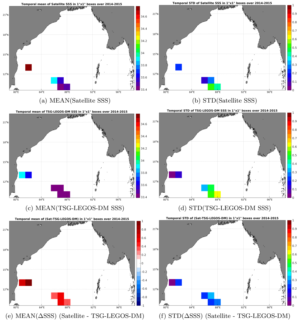
Figure 6: Temporal mean (left) and STD (right) of SSS from AQUARIUS-L2-JPL-V4 (top), TSG-LEGOS-DM (middle), and of \Delta SSS (Satellite - TSG-LEGOS-DM). Only match-up pairs are used to generate these maps.
