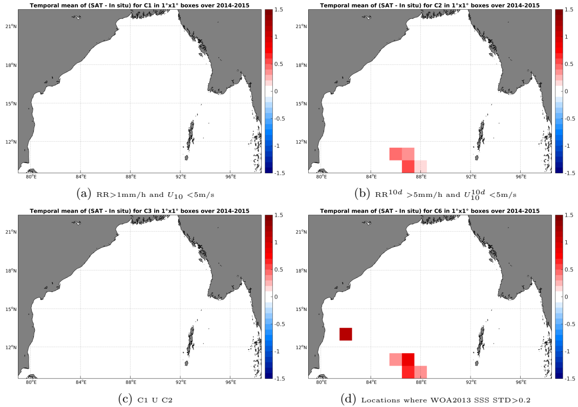
Figure 12: Temporal mean gridded over spatial boxes of size 1^\circ \times 1^\circ of \Delta SSS (AQUARIUS-L2-JPL-V4 - TSG-LEGOS-DM) for 4 different subdatasets corresponding to:RR >1 mm/h and U_{10} < 5 m/s (a), RR 10d > 5 mm/h and U_{10}^{10d} < 5 m/s (b), C1 U C2 (c),Locations where WOA2013 SSS STD >0.2 (d).
