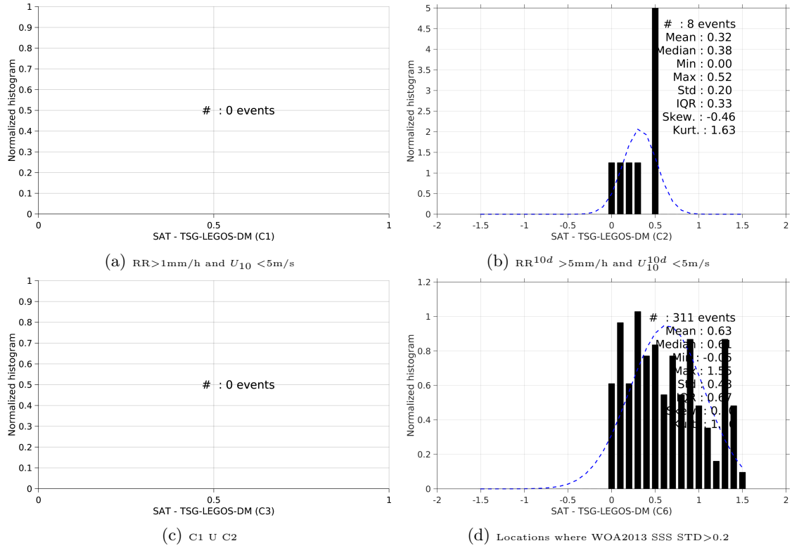
Figure 13: Normalized histogram of \Delta\text{SSS} (AQUARIUS-L2-JPL-V4 - TSG-LEGOS-DM) for 6 different subdatasets corresponding to: RR > 1\text{mm/h} and U_{10} < 5\text{m/s} (a), RR^{10d} > 5\text{mm/h} and U_{10}^{10d} < 5\text{m/s} (b), C1 \cup C2 (c), Locations where WOA2013 SSS STD > 0.2 (d).
