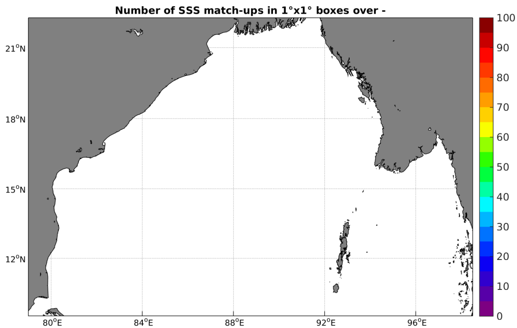
Figure 4: Number of SSS match-ups between TSG-GOSUD-Research-vessel SSS and the AQUARIUS-L2-JPL-V4 SSS product for the Bay of Bengal Pi-MEP region over 1°x1° boxes and for the full satellite product period.
