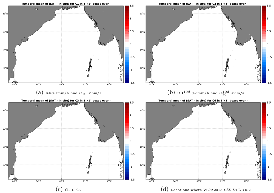
Figure 12: Temporal mean gridded over spatial boxes of size 1^\circ \times 1^\circ of \Delta SSS (AQUARIUS-L2-JPL-V4 - TSG-GOSUD-Research-vessel) for 4 different subdatasets corresponding to:RR >1 mm/h and U_{10} < 5 m/s (a), RR ^{10d} > 5 mm/h and U_{10}^{10d} < 5 m/s (b), C1 U C2 (c),Locations where WOA2013 SSS STD >0.2 (d).
