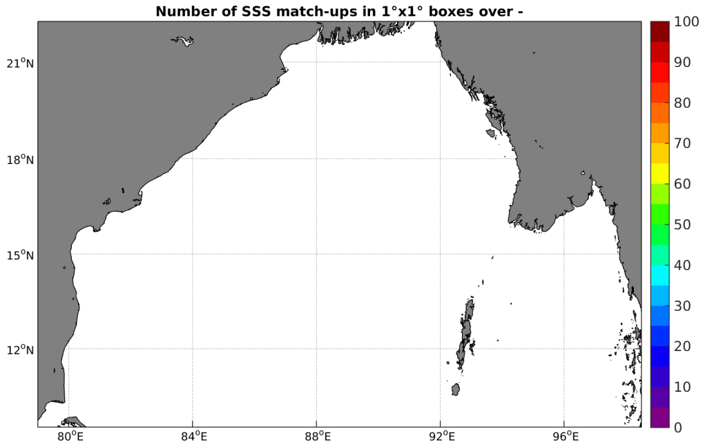
Figure 4: Number of SSS match-ups between Sea mammals SSS and the AQUARIUS-L2-JPL-V4 SSS product for the Bay of Bengal Pi-MEP region over 1^\circ \times 1^\circ boxes and for the full satellite product period.
