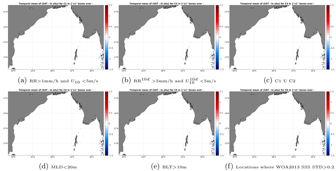
Figure 12: Temporal mean gridded over spatial boxes of size 1^\circ \times 1^\circ of \Delta SSS (AQUARIUS-L2-JPL-V4 - Sea mammals) for 6 different subdatasets corresponding to:RR>1mm/h and U_{10} < 5\text{m/s} (a), RR^{10d} > 5\text{mm/h} and U_{10}^{10d} < 5\text{m/s} (b), C1 U C2 (c),MLD<20m (d),BLT>10m (e),Locations where WOA2013 SSS STD>0.2 (f).
