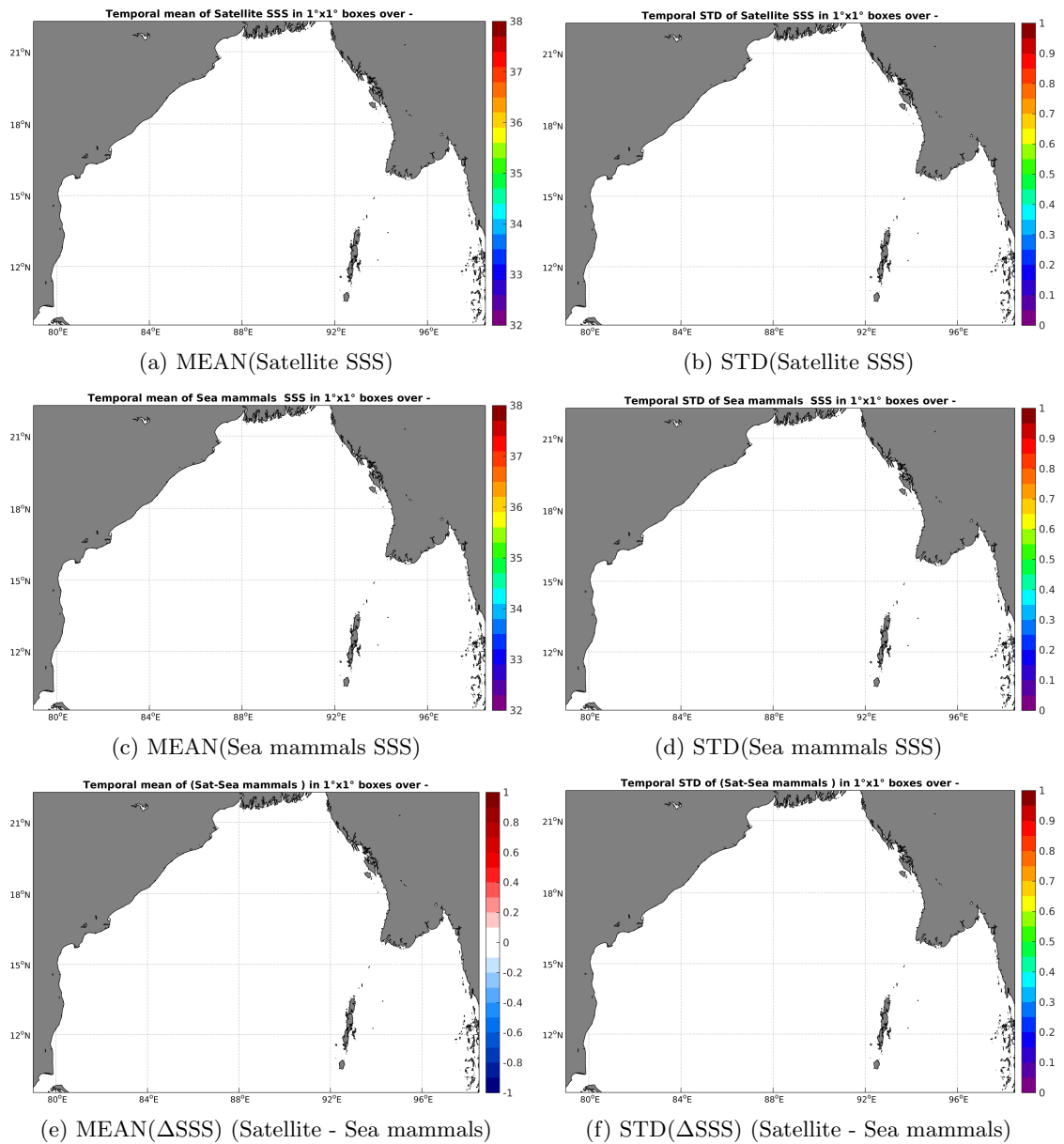
Figure 6: Temporal mean (left) and STD (right) of SSS from AQUARIUS-L2-JPL-V4 (top), Sea mammals (middle), and of \Delta SSS (Satellite - Sea mammals). Only match-up pairs are used to generate these maps.
