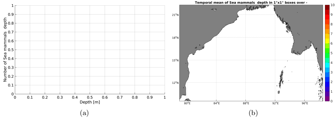
Figure 3: Histograms of the depth of the upper level SSS measurements from Sea mammals in the Match-up DataBase for the Bay of Bengal Pi-MEP region (a) and temporal mean spatial distribution of pressure of the in situ SSS data over 1^\circ \times 1^\circ boxes and for the full satellite product period (b).
