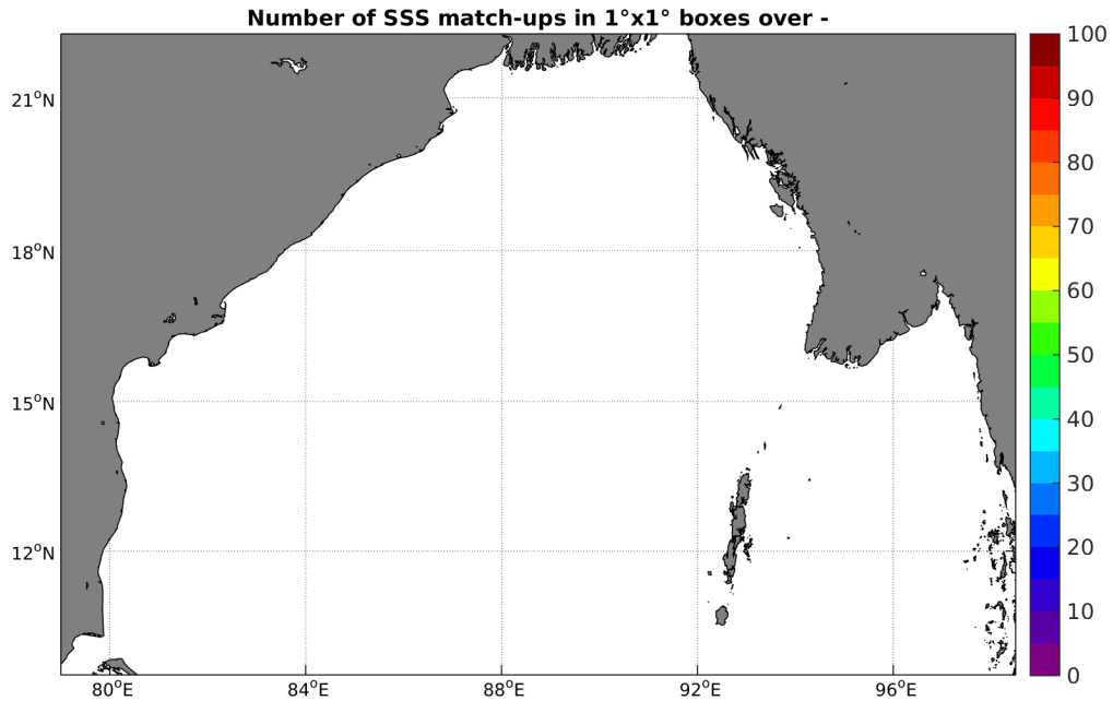
Figure 3: Number of SSS match-ups between Surface drifters SSS and the AQUARIUS-L2-JPL-V4 SSS product for the Bay of Bengal Pi-MEP region over 1°x1° boxes and for the full satellite product period.
