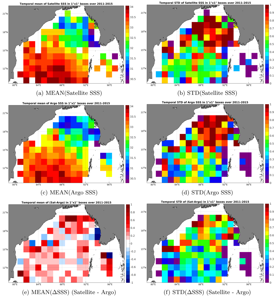
Figure 6: Temporal mean (left) and STD (right) of SSS from AQUARIUS-L2-JPL-V4 (top), Argo (middle), and of \Delta SSS (Satellite - Argo). Only match-up pairs are used to generate these maps.
