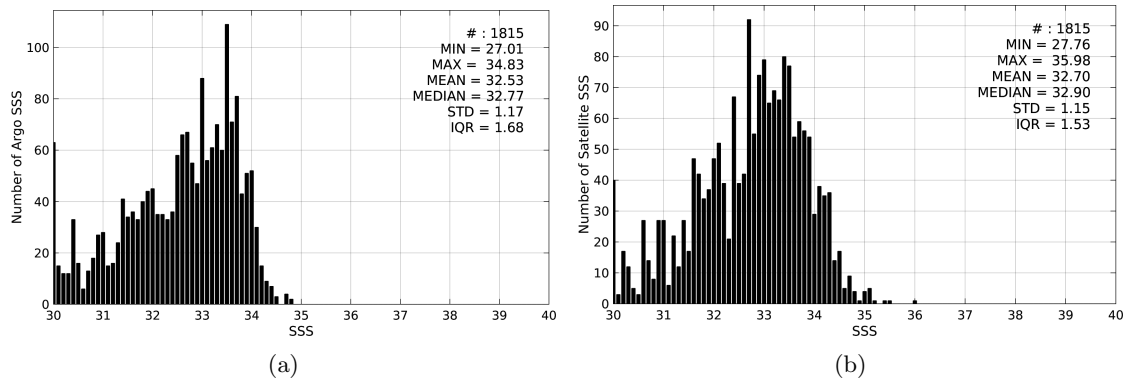
Figure 2: Histograms of SSS from Argo (a) and AQUARIUS-L2-JPL-V4 (b) considering all match-up pairs per bins of 0.1 over the Bay of Bengal Pi-MEP region and for the full satellite product period.
