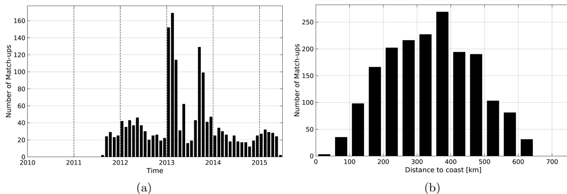
Figure 1: Number of match-ups between Argo and AQUARIUS-L2-JPL-V4 SSS as a function of time (a) and as function of the distance to coast (b) over the Bay of Bengal Pi-MEP region and for the full satellite product period.
