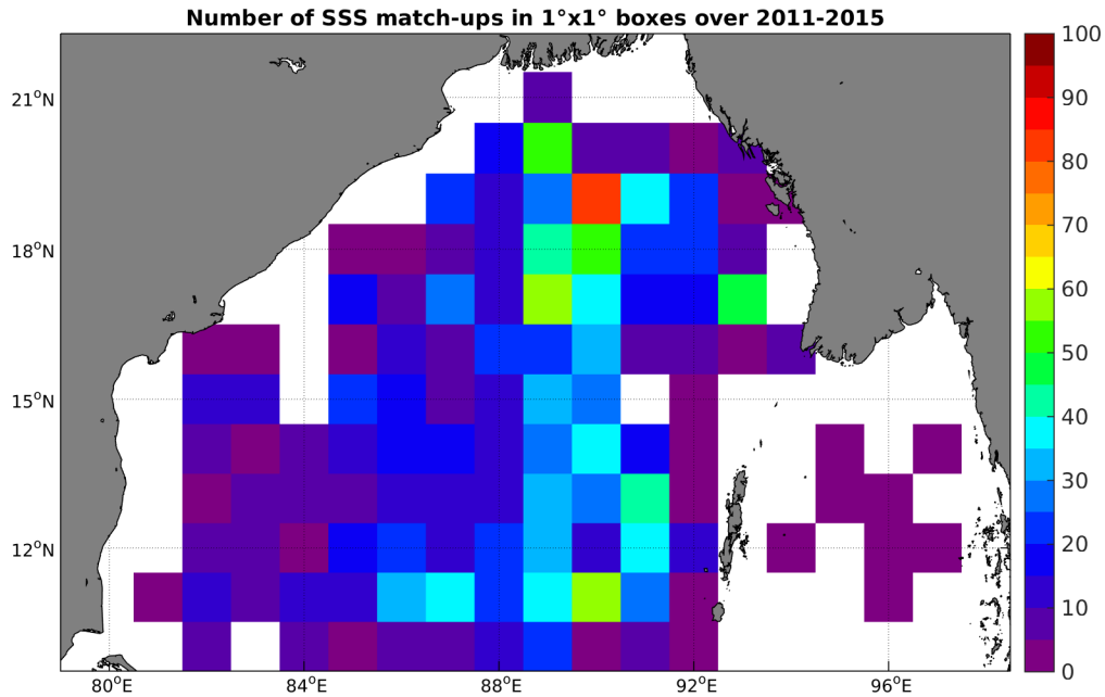
Figure 4: Number of SSS match-ups between Argo SSS and the AQUARIUS-L2-JPL-V4 SSS product for the Bay of Bengal Pi-MEP region over 1^\circ \times 1^\circ boxes and for the full satellite product period.
