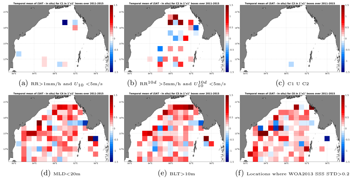
Figure 12: Temporal mean gridded over spatial boxes of size 1^\circ \times 1^\circ of \Delta\text{SSS} (AQUARIUS-L2-JPL-V4 - Argo) for 6 different subdatasets corresponding to: \text{RR} > 1\text{mm/h} and U_{10} < 5\text{m/s} (a), \text{RR}^{10d} > 5\text{mm/h} and U_{10}^{10d} < 5\text{m/s} (b), C1 U C2 (c), \text{MLD} < 20\text{m} (d), \text{BLT} > 10\text{m} (e), Locations where WOA2013 SSS STD > 0.2 (f).
